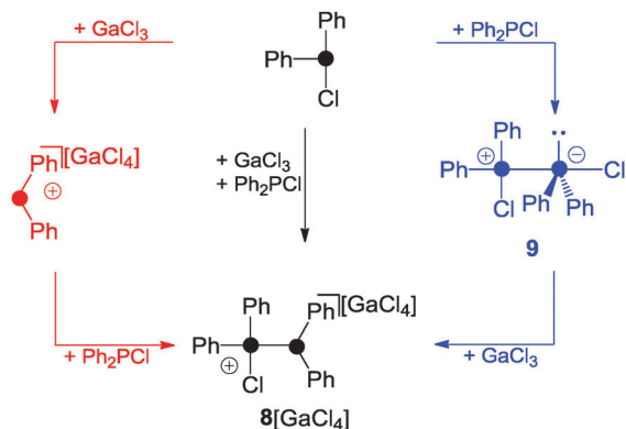
Scheme 1 Synthesis of 8[GaCl_4] by the reaction of Ph_2P(Ph)Cl and GaCl_3 in 2:1 stoichiometry and possible reaction sequences giving 8[GaCl_4] either via free Ph_2P^+ -phosphonium ion (red) or zwitterion 9 (blue).
