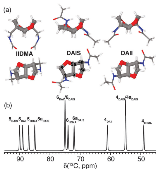
Fig. 6 (a) Top and side views of the most stable conformers for the primary diamines isodide-2,5-dimethyleneamine (IIDMA, endo-endo ), diaminoisosorbide (DAIS, exo-endo ), and diaminoisoidide (DAII, exo-exo ) found via gas phase MP2/6-311G** calculations. (b) Graphical representation of the calculated ^{13}\text{C} chemical shifts for all three conformers assigned using the nomenclature shown for DAIS in (a). Reprinted with permission from ref. 75. Copyright 2012, American Chemical Society.
