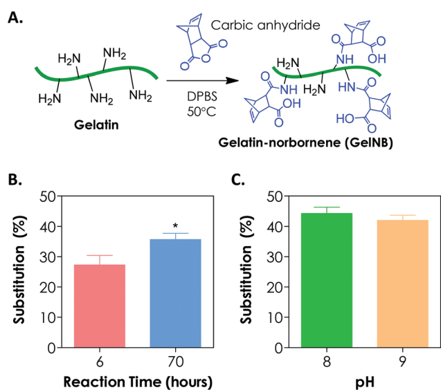
Fig. 1 (A) Schematic of gelatin-norbornene (GelNB) synthesis. (B) Effect of reaction time (without pH adjustment) on the degree of norbornene substitution (* p < 0.05). (C) Effect of the solution pH value on the degree of norbornene substitution. In all reactions, carbic anhydride was added at 20 wt/vol%.
