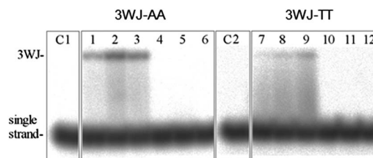
Fig. 10 Autoradiograms of the gels run at room temperature. Lane C1: control containing the three strands, S1-AA, S2 and S3. Lanes 1–3: S1-AA, S2 and S3 mixed with \Lambda_{Fe}/S_C-[Fe_2L^{1a}_3]Cl_4 at 0.5 : 1, 1 : 1 and 2 : 1 (flexicate : 3WJ) ratios, respectively. Lanes 4–6: S1-AA, S2 and S3 mixed with \Delta_{Fe}/R_C-[Fe_2L^{1a}_3]Cl_4 at 0.5 : 1, 1 : 1 and 2 : 1 (flexicate : 3WJ) ratios, respectively. Lane C2: control containing the three strands, S1-TT, S2 and S3. Lanes 7–9: S1-TT, S2 and S3 mixed with \Lambda_{Fe}/S_C-[Fe_2L^{1a}_3]Cl_4 at 0.5 : 1, 1 : 1 and 2 : 1 (flexicate : 3WJ) ratios, respectively. Lanes 10–12: S1-TT, S2 and S3 mixed with \Delta_{Fe}/R_C-[Fe_2L^{1a}_3]Cl_4 at 0.5 : 1, 1 : 1 and 2 : 1 (flexicate : 3WJ) ratios, respectively.
