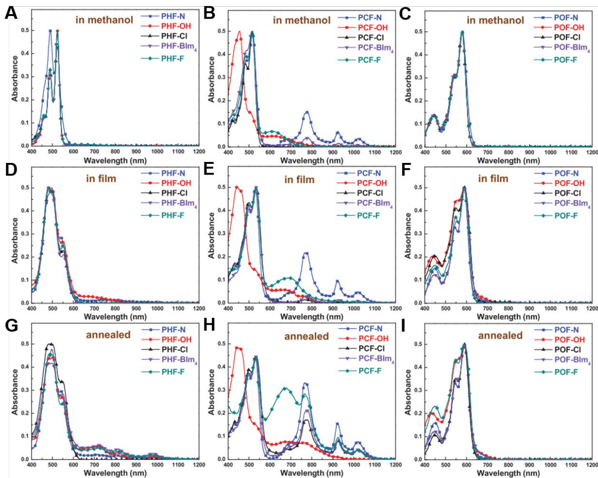
Figure 9. Absorption spectra of P'R'F-'X' derivatives ( A-C ) in methanol, ( D-F ) as cast in thin films, and ( G-I ) after annealing at 85°C for 20 min. Reprinted with permission from ref 128. Copyright 2017 John Wiley & Sons Inc.
