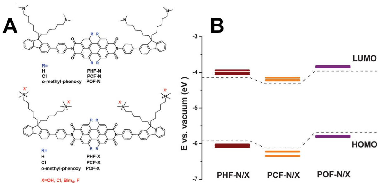
Figure 8. (A) Chemical structures of P'R'F-'X' derivatives, where R corresponds to bay functionalization with hydrogen, chlorine, or o-methyl-phenoxy, and X corresponds to the anionic counterion in quaternary ammonium structures, where OH is hydroxyl, Cl chloride, BIm 4 is tetrakis(1-imidazolyl)borate, and F is fluoride. (B) Relative changes to the HOMO/LUMO levels when the PDI core is functionalized with hydrogen, chlorine, or o-methyl-phenoxy in PHF-X, PCF-X, and POF-X, respectively. Reprinted with permission from ref 128. Copyright 2017 John Wiley & Sons Inc.
