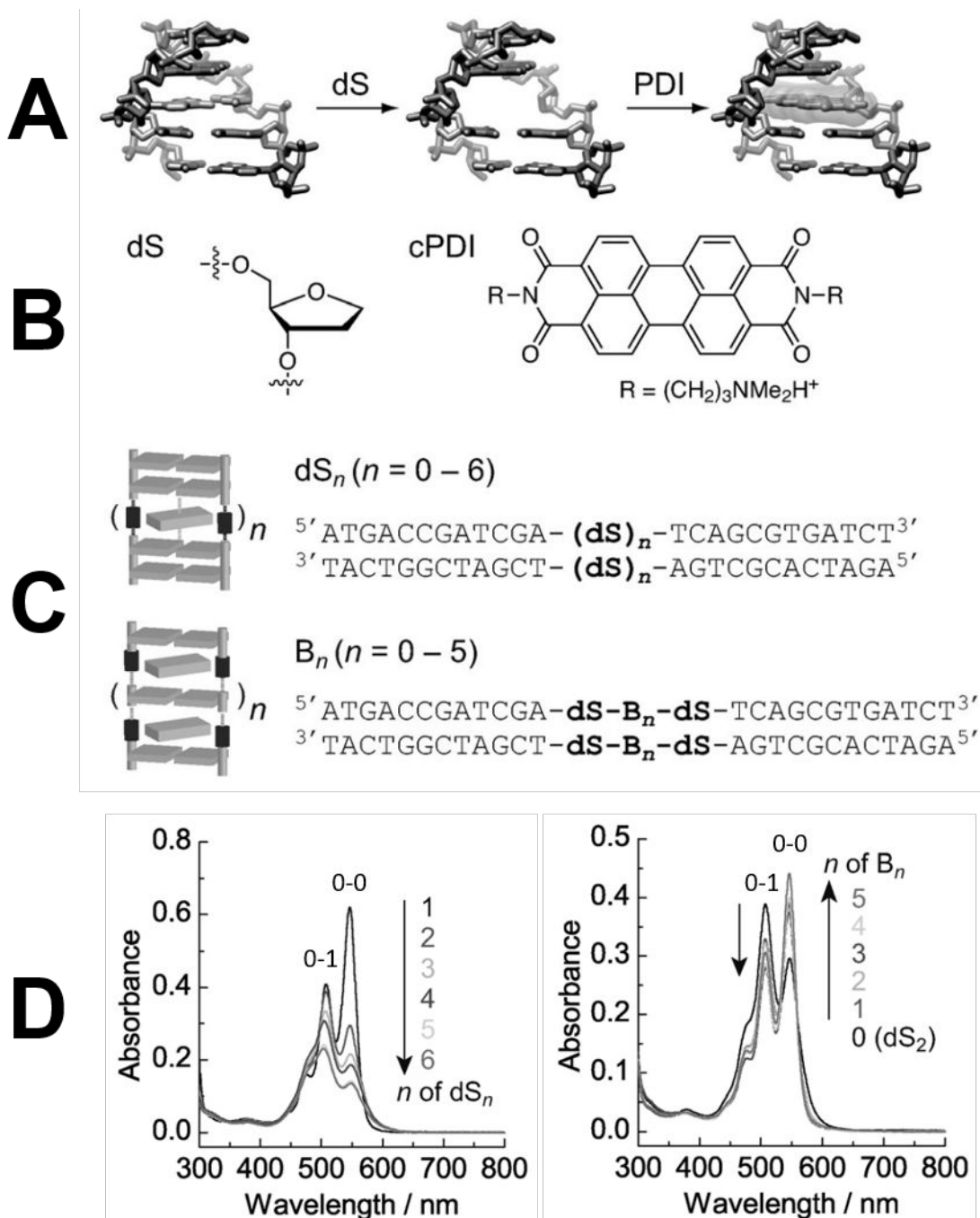
Figure 12. (A) Representation of PDI coordinating to a hydrophobic pocket created within a DNA strand by replacing nucleosides with abasic analogues. (B) Structure of the abasic deoxyribose spacer (dS) and cPDI. (C) DNA sequences with different binding cavity configurations; the first with dS_n abasic sites and the second with B_n cavity spacers composed of alternating A-T pairs
