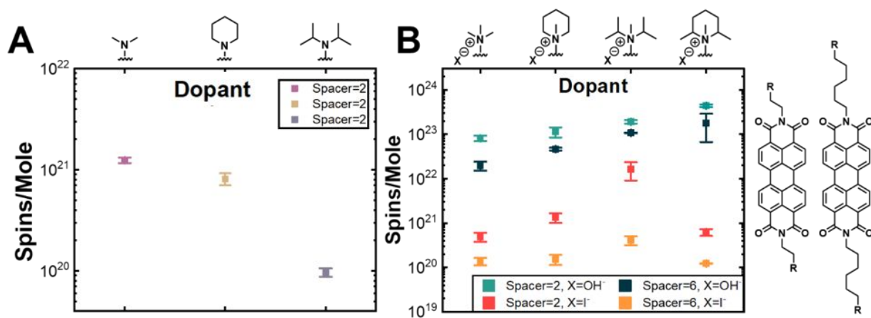
Figure 10. (A) Quantitative EPR measurements of spin concentration for tertiary amino doped N-PDIs with increasing steric encumbrance. (B) Quantitative EPR of sterically encumbered ammonium doped N-PDIs. The groups vary by steric encumbrance, tether length, and counterion.
