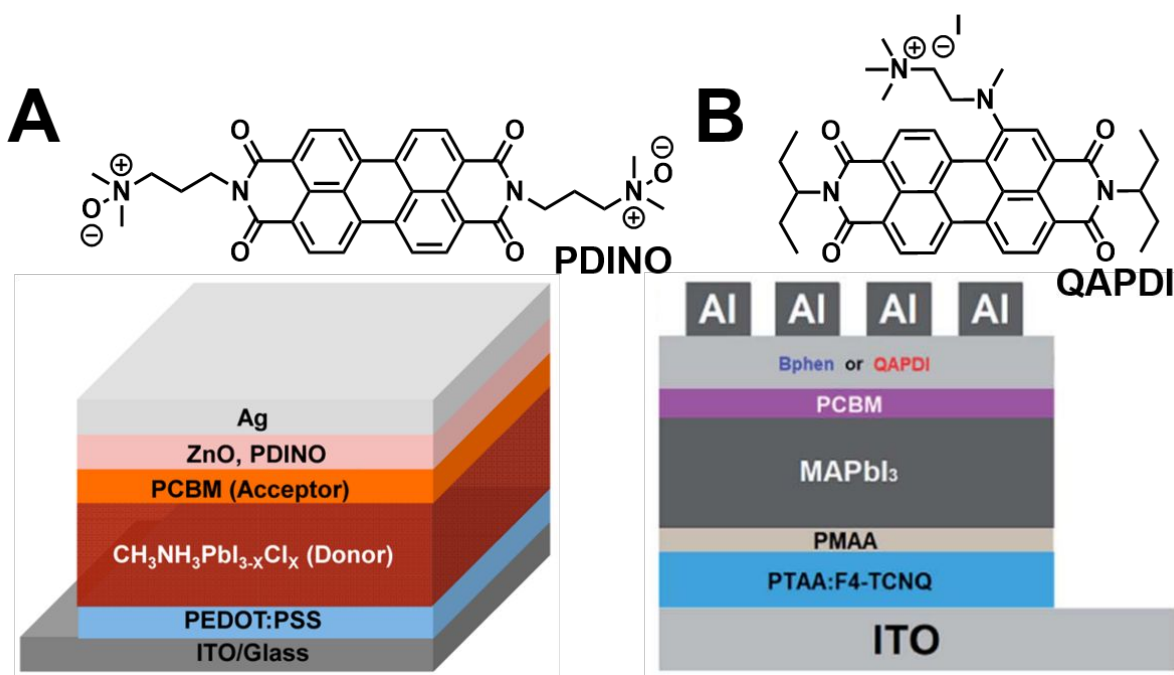
Figure 17. (A) Chemical structure of PDINO and the relevant corresponding device stack. Reprinted with permission from ref. 206. Copyright 2015 American Chemical Society. (B) Structure of QAPDI and the relevant corresponding device stack. Reproduced from ref. 206. Copyright 2020 The Royal Society of Chemistry.
