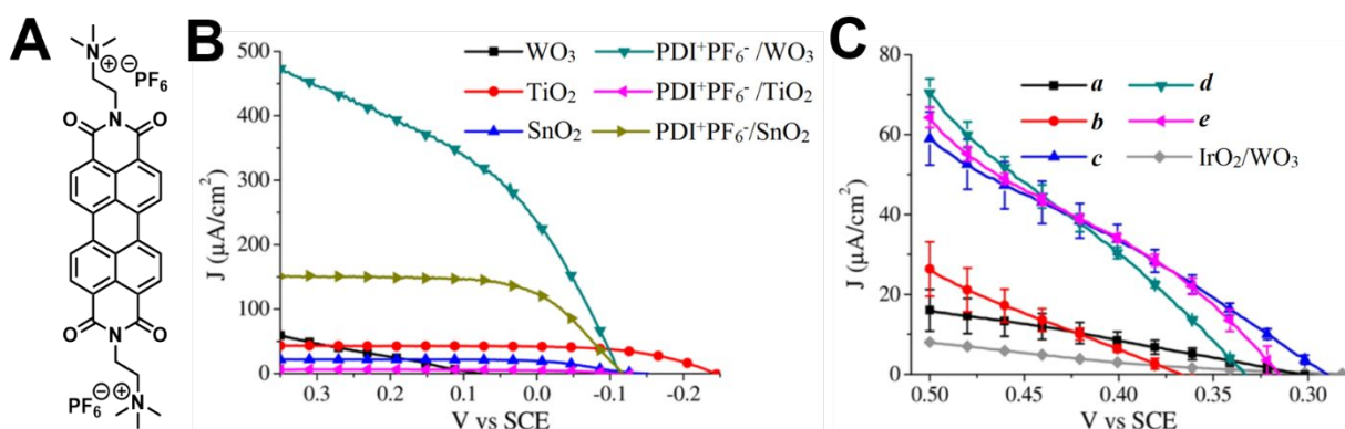
Figure 20. (A) Chemical structure of PDI+PF 6 - . (B) J – V curves of electrodes with and without the application of the PDI+PF 6 - sensitizer in the presence of acetonitrile/0.1 M LiI. The current densities shown are obtained by subtracting their respective dark currents. (C) J – V curves of different batches of PDI+PF 6 - /WO 3 photoelectrodes with (b–e) and without (a) and IrO 2 modifier. Reprinted with permission from ref. 58. Copyright 2015 American Chemical Society.
