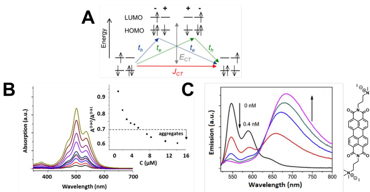
Figure 3. (A) Energy level diagram of charge-transfer coupled chromophores. Reprinted with permission from ref. 75. Copyright 2017 American Chemical Society. (B) Prototypical concentration-dependent (1-14 \mu\text{M} ) absorption spectra of a PDI in water exhibiting H-type aggregate formation. Peak area ratios of the 0-0/0-1 vibronic peaks are shown in the inset. Reprinted with permission from ref. 76. Copyright 2017 Elsevier. (C) Emission spectra of QA-I (right) titrated with 0-0.4 nM Ag nanoparticles. The nanoparticles induce PDI excimer formation at elevated concentrations. Reprinted with permission from ref. 80. Copyright 2018 Elsevier.
