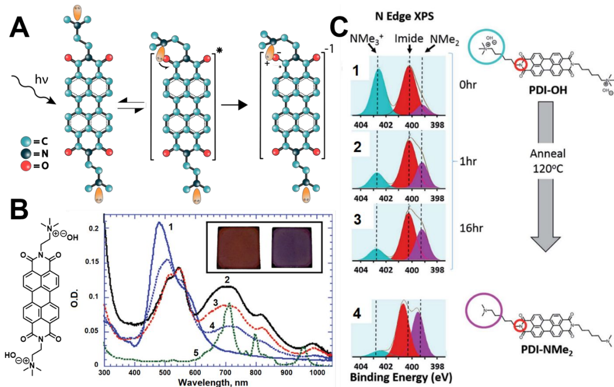
Figure 4. (A) A graphical representation of the self-n-doping mechanism. (B) Chemical structure of the compound analyzed in the accompanying absorption spectrum. The numbered spectra correspond to the absorption of the (1) as cast; (2) after heating at 120 °C for 20 min in air; (3) 10 min after exposure to ~33% humidity air; (4) 24 h in ambient air; (5) electrochemically generated radical anion in THF. Inset: as-cast film (left) and heated film (right). Adapted with permission from ref 55. Copyright 2012 John Wiley & Sons Inc. (C) N 1s XPS spectra of an N-PDI (PDI-OH) before (1) and after heating at 120 °C for 1 h (2) and 16 h (3), as well as the N 1s XPS spectrum of the (PDI-NMe 2 ) for reference (4). The relative peak ratios of NMe 3 + , imide, and NMe 2 are shown in blue, red, and purple, respectively. Adapted with permission from ref 127. Copyright 2012 John Wiley & Sons Inc.
