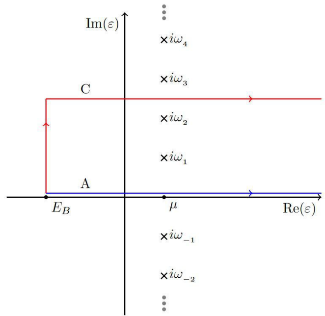
Fig. 6 The contour labeled C is used for integration of the Green's function defining the core-lifetime broadened XAS as well as the electron density. Reprinted figure with permission from [T. S. Tan, J. Kas and J. Rehr, Physical Review B , 104, 035144 (2021)], Copyright (2022) by the American Physical Society.
