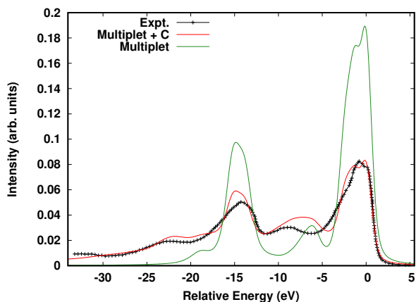
Fig. 12 Fe 2p XPS of \alpha Fe 2 O 3 calculated within the multiple+C approach (red) compared to the multiplet-only spectrum (green), and experimental results (black crosses). Reprinted figure with permission from [J. J. Kas, J. J. Rehr and T. P. Devereaux, Ab initio multiplet plus cumulant approach for correlation effects in x-ray photoelectron spectroscopy, 2021, https://arxiv.org/abs/2107.10409 ]
