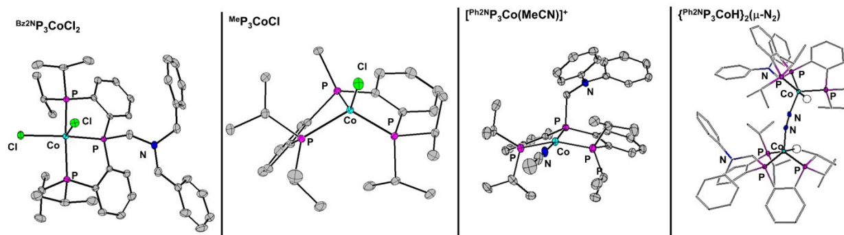
Figure 1. 50% Thermal ellipsoid plot of several complexes. All hydrogen atoms not located in the difference map are removed for clarity. Only the cation of [(\text{Ph}_2\text{NP}_3\text{Co}(\text{MeCN}))][\text{BARF}] is shown.
