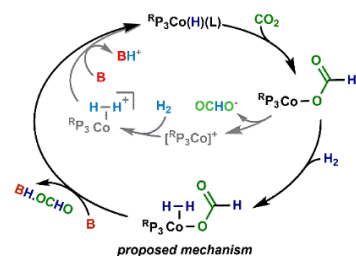
Scheme 1. Proposed mechanism for hydrogenation of CO_2 to formate, with alternate mechanism shown in grey.
