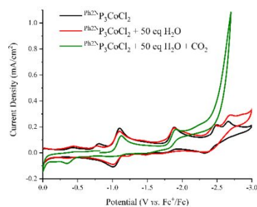
Figure 3. Cyclic voltammograms of 1 mM Ph^2NP_3CoCl_2 under various conditions. (black): under N_2 ; (red): in the presence of 50 eq H_2O ; (green): in the presence of 50 eq H_2O and CO_2 . Conditions: GC working electrode, 0.1 M TBAPF 6 electrolyte in MeCN solvent, scan rate of 0.06 V/s, initial scan is positive
