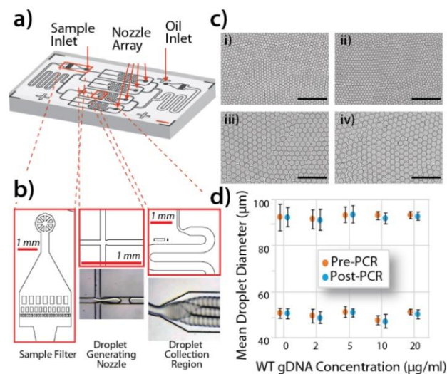
Figure 2. High-throughput droplet generation and thermocycling stability. A) Schematic of custom droplet generation chip with inlets and outlets identified. B) Close-up view of three important features including: integrated sample and oil filter, droplet generating nozzle array (flow-focusing principle), and droplet collection region. C) Brightfield microscope images of a 2D monolayer of droplets in a hemocytometer, i) 50 \mu\text{m} droplets pre-PCR, ii) 50 \mu\text{m} droplets post-PCR, iii) 90 \mu\text{m} droplets pre-PCR, iv) 90 \mu\text{m} droplets post-PCR. Scale bar = 500 \mu\text{m} . D) Quantitative measurements of individual droplet diameters demonstrate robust droplet stability before and after thermocycling across a range of gDNA concentrations from 0–20 \mu\text{g}/\text{ml} .
