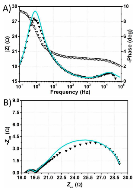
Figure 8. Phase (filled triangles) and modulus (open triangles) Bode (A) and Nyquist (B) plots of the dummy cell filled with aqueous electrolyte comprised of NaI 1.50 M + I_2 50 mM. Data points were fitted (light blue lines) according to Eq. 1.
