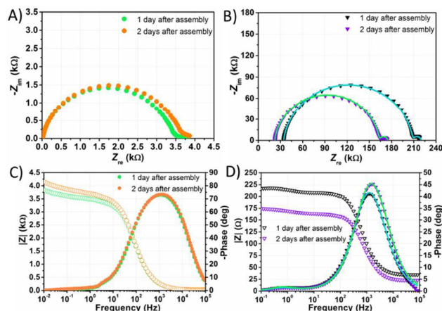
Figure 7. EIS spectra of aqueous DSSCs assembled with KI 1.50 M + I_2 50 mM (A,C) and NaI 1.50 M + I_2 50 mM (B,D). Data points were fitted (lines) according to Eq. 3 with the constraints R_{Pt} = 2 \Omega and C_{Pt} = 2 \times 10^{-5} F .
