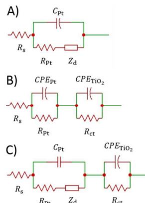
Figure 2. Equivalent circuits proposed for the EIS investigation of aqueous devices under study.
