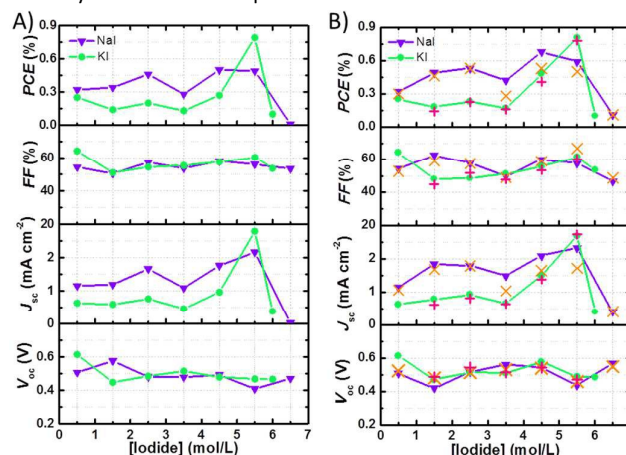
Figure 4. Photovoltaic parameters (A = after 24 h from cell assembly, B = best value recorded in the cell lifetime) of aqueous DSSCs bearing different I^- concentrations ( I_2 50 mM). Orange crosses (X) or red plus (+) stand for the average values at the given NaI or KI concentrations, respectively. Lines just connect data points and have no physical meaning. Cells were tested under 1 sun irradiation and the reported data were recorded at the 3 rd J-V measurement.
