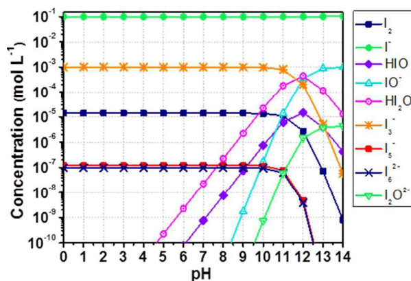
Figure 1. Computed concentration of iodine compounds in a solution containing aqueous I^- 0.10 M and I_2 1.0 mM as a function of the pH. Results are computed as described in this section, comparable with those obtained by Gottardi (see Figure S1). 31 Lines just connect data points for better reading and have no physical meaning.
