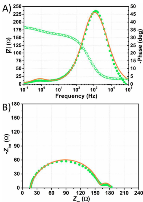
Figure 9. Phase (filled circles) and modulus (open circles) Bode (A) and Nyquist (B) plots of the dummy cell filled with aqueous electrolyte comprised of KI 1.50 M + I_2 50 mM. Data points, recorded 5 months after cell assembly, were fitted (lines) according to Eq. 3 with the constraint R_{pt} = 2 \Omega and C_{pt} = 2 \times 10^{-5} \text{ F} .
