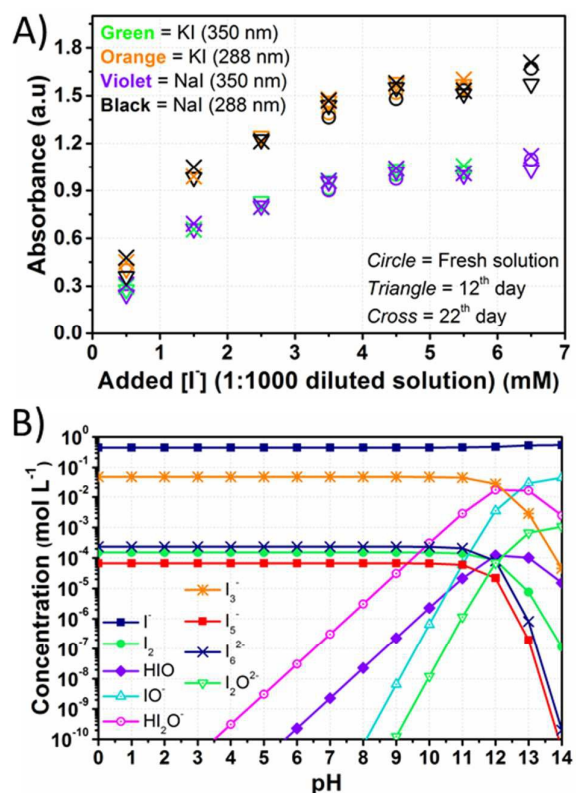
Figure 6. A) Intensity of the peaks of \text{IO}_3^- in the UV region plotted versus the amount of \text{I}^- in the solutions obtained by diluting at 1:1000 the stock aqueous electrolytes containing \text{I}_2 50 mM and different amounts of iodine salts; B) Computed equilibrium concentrations for electrolytes containing \text{I}^- 0.50 M + \text{I}_2 50 mM considering the reactions listed in Table S4. Lines just connect data points for better reading and have no physical meaning.
