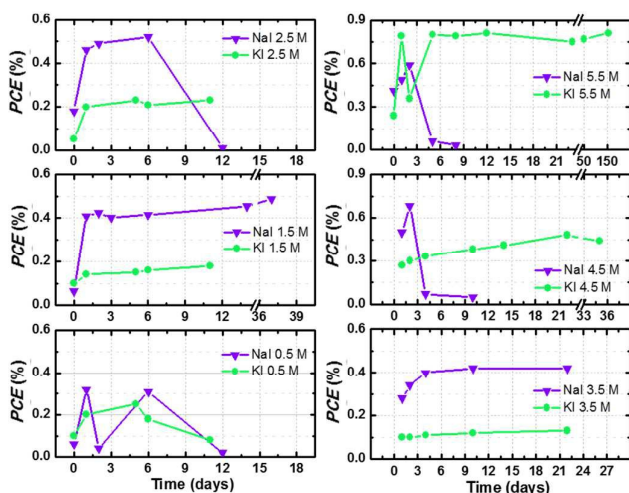
Figure 5. PCE values upon time of aqueous DSSCs assembled with different I - salts and at different concentrations, keeping constant I 2 at 50 mM. Cells (stored at room temperature under dark conditions) were tested at 1 sun irradiation and the reported data were recorded at the 3 rd J-V measurement. Lines just connect data points for better reading and have no physical meaning.
