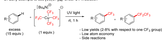
C: Neutral Cu(III) reagents in trifluoromethylation
