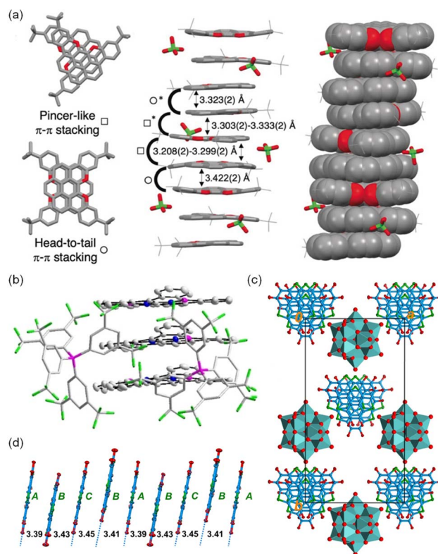
Fig. 20 (a) \pi - \pi stacking in the crystal structure of 60b_3(\text{ClO}_4)_2 \cdot \text{THF} \cdot (\text{H}_2\text{O})_{0.5} ; (b) \pi -stacked trimer in the crystal structure of 61b_3^{2(+)}(\text{BAR}_4^{\text{F}-})_2 ; (c) a unit cell in the crystal structure of 62a_4^{3+}(\text{PMo}_{12}\text{O}_{40})^{3-} ; (d) \pi - \pi stacking in the crystal structure of 62a_4^{3+}(\text{PMo}_{12}\text{O}_{40})^{3-} . Reproduced with permission from ref. 110–112. Copyright 2020, 2023 and 2024 Wiley.
