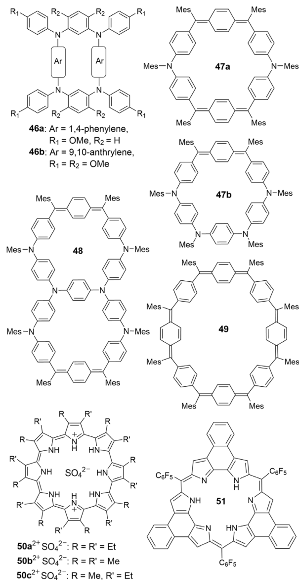
Fig. 15 Conjugated macrocycles that afford multiple radical cations.
