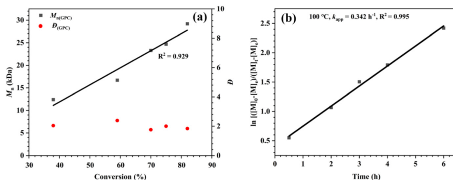
Fig. 1 (a) M_n and \bar{D} of the resultant PDDL versus monomer conversion ( [M]_0/[I]_0/[C]_0 = 100/1/1 , [M]_0 = \text{bulk} , T = 100 °C). (b) Kinetic plots of \ln\{([M]_0 - [M]_e)/([M]_t - [M]_e)\} vs. time ( [M]_0/[I]_0/[C]_0 = 100/1/1 , [M]_0 = \text{bulk} , T = 100 °C) of DDL.
