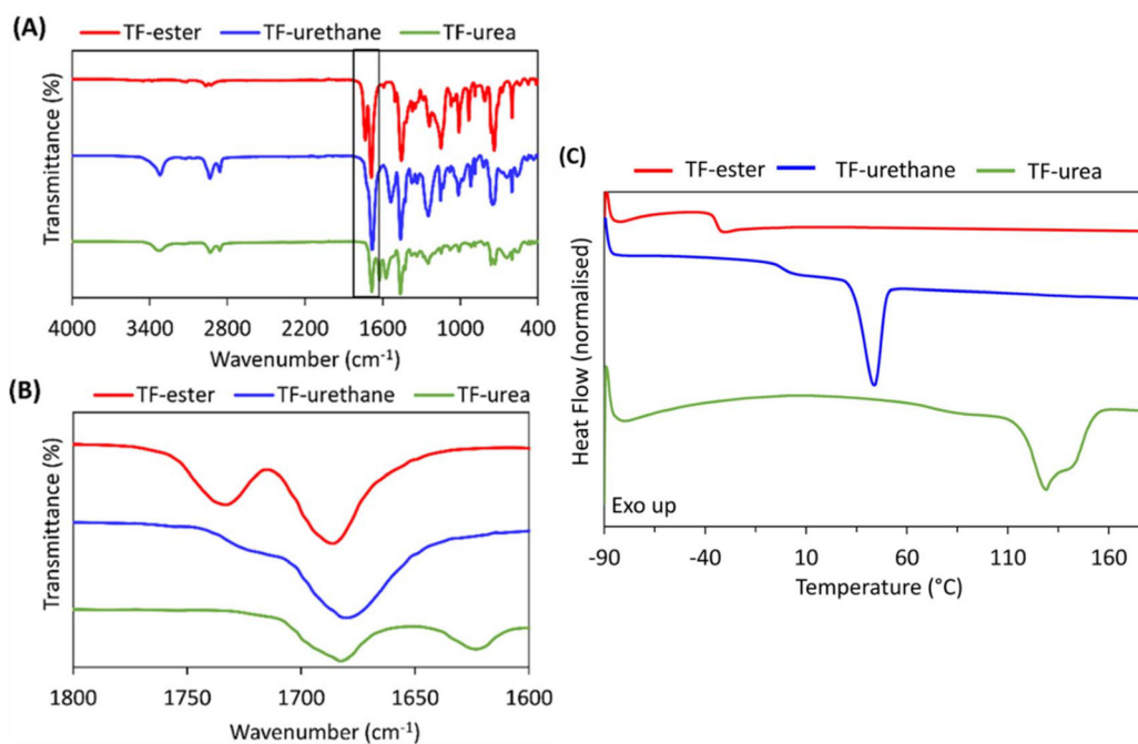
Fig. 1 (A) ATR-FTIR spectra of TF crosslinkers, (B) ATR-FTIR spectra of TF-crosslinkers zoomed into the carbonyl region and (C) DSC thermograms (1st heating cycles) of TF crosslinkers.
