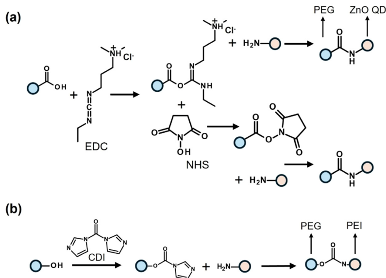
Fig. 4 (a) Chemical reaction scheme of EDC/NHS coupling of a carboxyl group on the ligand (bioactive compound) to a primary amine on the bioactive compound (ligand). (b) N,N' -Carbonyldiimidazole (CDI)-mediated coupling of a hydroxyl group on the polyethylene glycol to a primary amine on the ligand.
