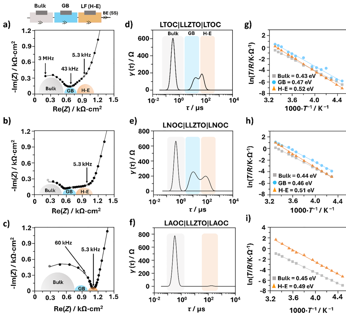
Fig. 3 Nyquist plots collected at 55 MPa and 25 °C for the bilayer symmetric LMOc|LLZTO|LMOc cells: (a) LTOC, (b) LNOC, (c) LAOC, and (d)–(f) the corresponding DRT maps. The hetero-electrolyte contribution observed at the lower frequency range (LF \approx 5 kHz) is denoted in orange; with the corresponding Arrhenius plots for (g) LTOC and (h) LNOC describing the activation energies for the bulk (HF), GB (MF) and H-E contributions, and (i) LAOC showing only the bulk (HF) and H-E (LF) contributions.
