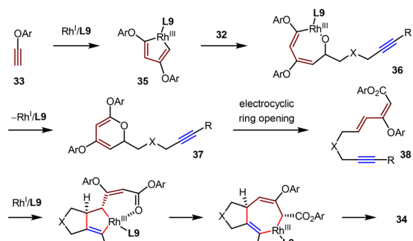
Scheme 12 \text{Rh}(\text{I})/(\text{R})\text{-H}_8\text{-BINAP} -catalyzed intermolecular [2+2+2] trimerization/asymmetric intramolecular [4+2] cycloaddition.
