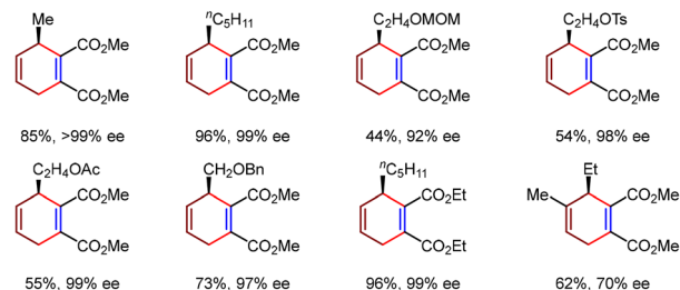
Scheme 13 \text{Rh}(\text{I}) /phosphoramidite-catalyzed asymmetric intermolecular [4+2] cycloadditions of 1,3-dienes and DMADs.
