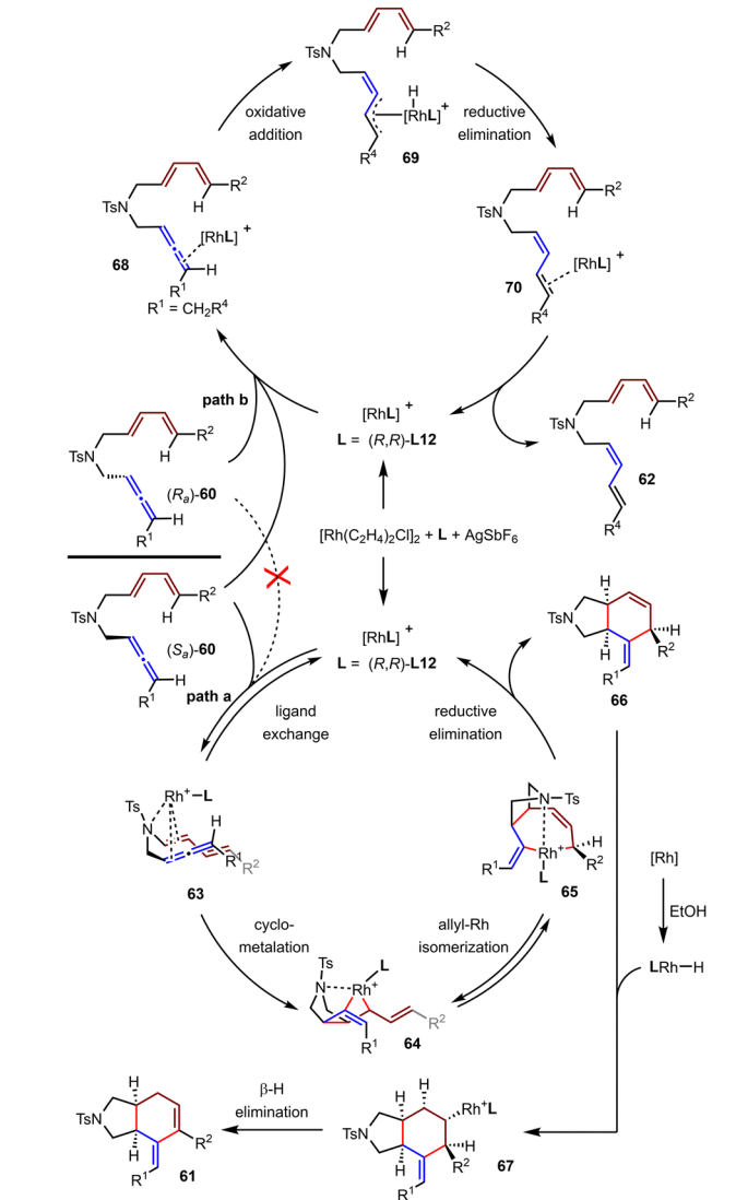
Scheme 18 Rh(i)/Ph-BPE-catalyzed kinetic resolution of racemic 1,3-disubstituted allenyl 1,3-dienes.
