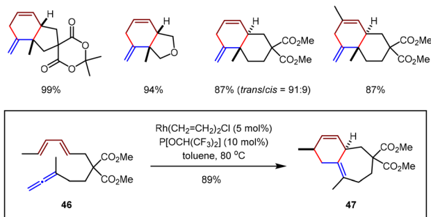
Scheme 14 \text{Rh}(\text{I}) /phosphite-catalyzed intramolecular [4+2] cycloaddition of 1,1-disubstituted allene-1,3-dienes.
