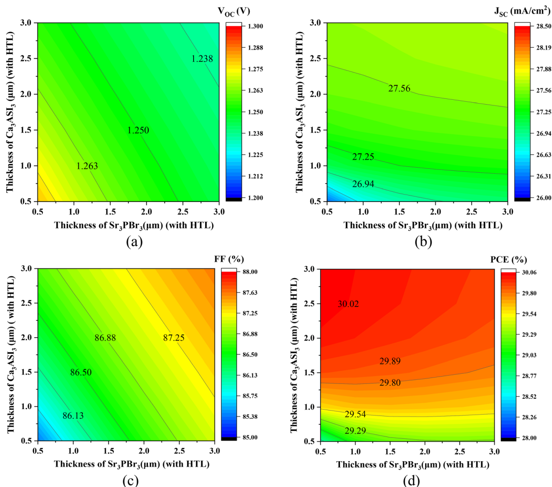
Fig. 4 Influence of thickness variation of \text{Sr}_3\text{PBr}_3 and \text{Ca}_3\text{AsI}_3 (device-iv) on the photovoltaic parameters, (a) V_{OC} , (b) J_{SC} , (c) FF , and (d) PCE .
