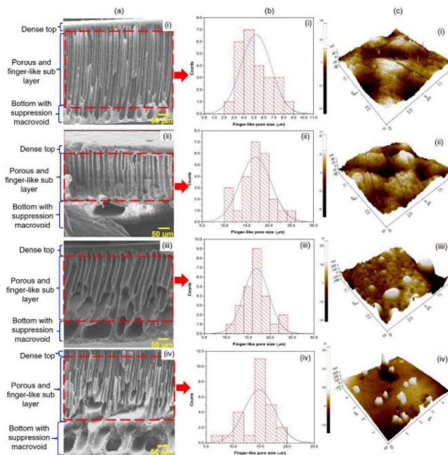
Fig. 6 (a) Cross-sectional images of SEM analysis. (b) Finger-like distribution of size of cavities. (c) AFM images of (i) PSf membrane and (ii) PSf-Ag/AgO membrane prepared using P. speciosa seeds, (iii) using pods and (iv) using leaves. 54
