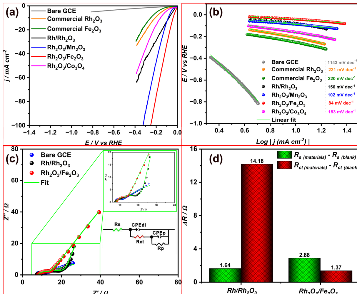
Fig. 5 (a) LSV curves recorded at a scan rate of 100 \text{ mV s}^{-1} for commercial \text{Rh}_2\text{O}_3 , commercial \alpha\text{-Fe}_2\text{O}_3 , and synthesized Rh/Rh _2\text{O}_3 , Rh _2\text{O}_3/\text{Mn}_2\text{O}_3 , Rh _2\text{O}_3/\text{Fe}_2\text{O}_3 , and Rh _2\text{O}_3/\text{Co}_3\text{O}_4 in 0.5 M \text{H}_2\text{SO}_4 (without iR compensation); (b) corresponding Tafel plots derived from the LSV data; (c) Nyquist plots for Rh/Rh _2\text{O}_3 , Rh _2\text{O}_3/\text{Fe}_2\text{O}_3 , and bare GCE, with insets showing magnified semicircle regions and the equivalent circuit used for fitting; (d) comparative plot of charge transfer resistance ( \Delta R_{\text{ct}} ) values extracted from EIS data for Rh/Rh _2\text{O}_3 and Rh _2\text{O}_3/\text{Fe}_2\text{O}_3 relative to bare GCE.
