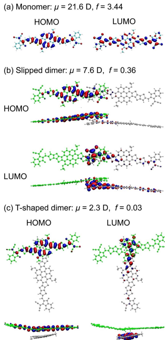
Fig. 4 Calculated transition dipole strength ( \mu ), oscillator strength ( f ), HOMO and LUMO (isovalue = 0.02) of (a) TACIC monomer, (b) slipped dimer, and (c) T-shaped dimer at the S_1 optimized geometry. The phenyl sidechains are omitted for simplicity.
