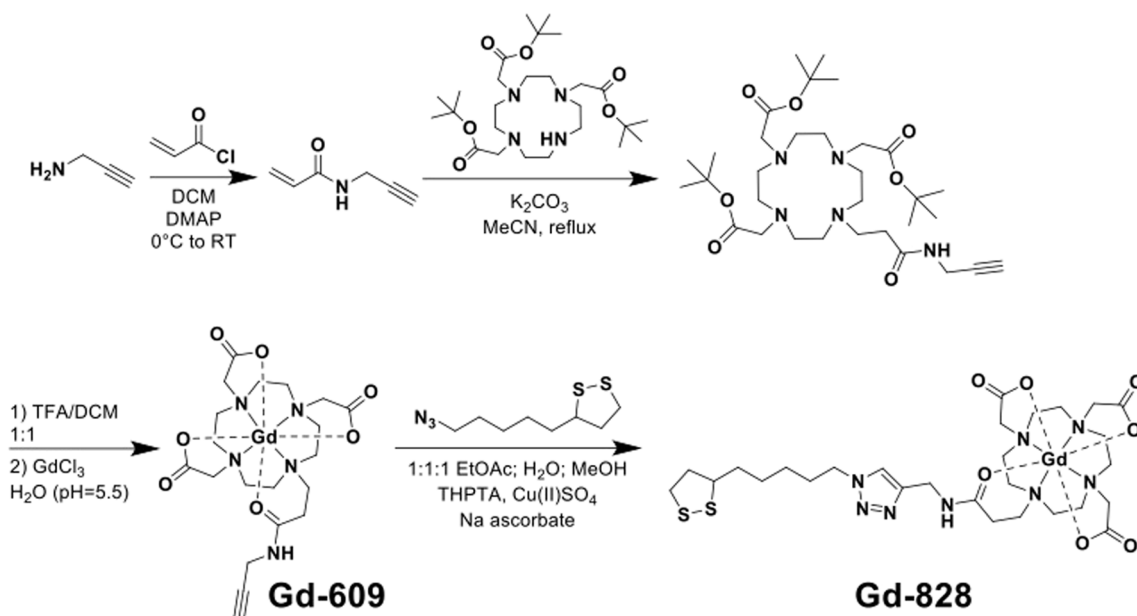
Scheme 1 Synthesis of small-molecule \text{Gd(III)} agents (Gd-609 and Gd-828).
