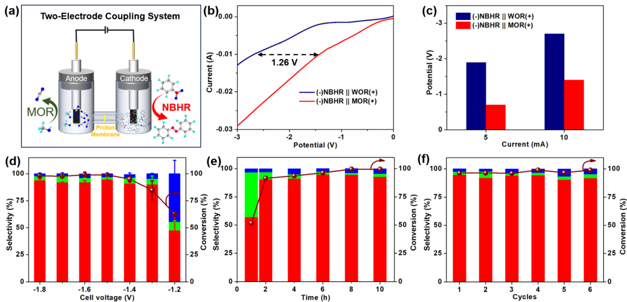
Fig. 5 Two-electrode coupling system. (a) A scheme illustrating the two-electrode coupling system with cathode NBHR and anode MOR. (b) LSV curves of PdS MNSSs in (-)\text{NBHR}||\text{MOR}(+) and (-)\text{NBHR}||\text{WOR}(+) . (c) Cell voltages of PdS MNSSs at different current densities in (-)\text{NBHR}||\text{MOR}(+) and (-)\text{NBHR}||\text{WOR}(+) . (d) Electrochemical selectivity and conversion of PdS MNSSs at different current densities in (-)\text{NBHR}||\text{MOR}(+) . (e) Time-dependent electrochemical selectivity and conversion of PdS MNSSs in (-)\text{NBHR}||\text{MOR}(+) ( -1.5 V). (f) Electrochemical stability of PdS MNSSs in (-)\text{NBHR}||\text{MOR}(+) ( -1.5 V).
