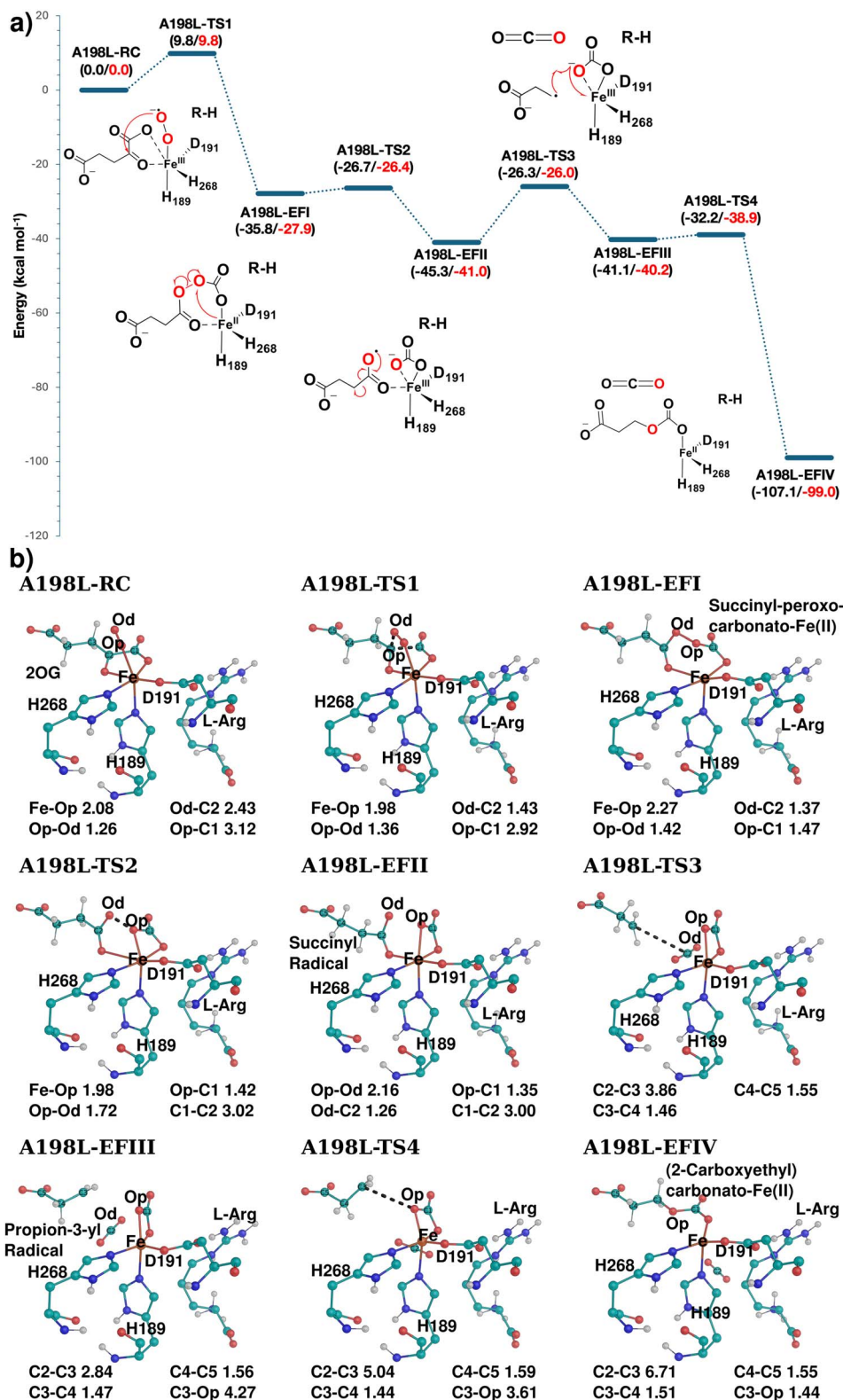
Fig. 7 (a) Reaction profile of the O 2 activation mechanism in the A198L-EFE variant. Relative energies are given in kcal mol -1 at QM(B2)/MM (black) and QM(B3)/MM (red) levels. The profile was plotted at the QM(B3)/MM level. (b) Optimized structures obtained during the QM/MM simulations. Distances are mentioned in Å.
