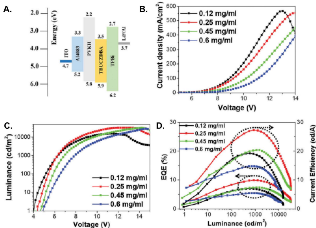
Fig. 82 Characterization of OLED device with different thicknesses of inkjet printed t BuCzDBA film as the active layer (A) device architecture and energy level diagram of the prepared OLEDs (B) current density versus voltage, (C) luminance versus voltage, and (D) efficiency versus luminance characteristics.
