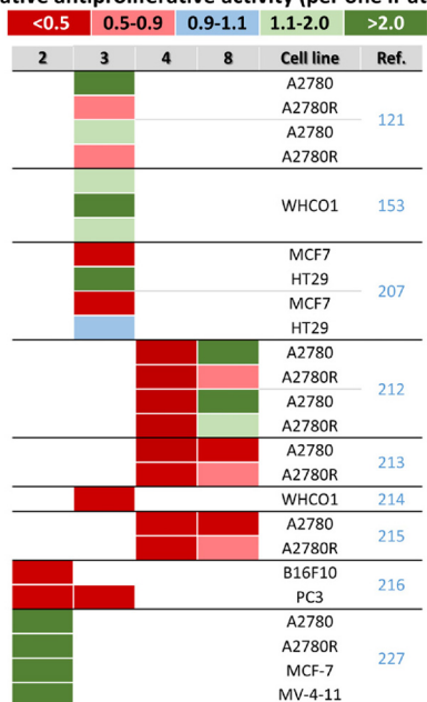
Fig. 37 A comparison of the antiproliferative activity of multinuclear Ir complexes ( n = 3, 4 or 8 ) and their mononuclear analogues; n stands for the number of Ir atoms. Relative activity (RA) = [\text{IC}_{50}(\text{mononuclear complex})]/[\text{IC}_{50}(\text{Ir multinuclear complex}) \times n] .
