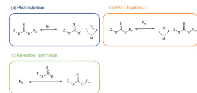
Scheme 1 General mechanism of PI-RAFT polymerisation. The S–C bond is photolysed to generate a free radical (a, photoactivation). The propagating radical can either chain transfer the active centre (b, RAFT equilibrium) or combine with a photoiniferter radical to terminate reversibly (c, reversible termination).
