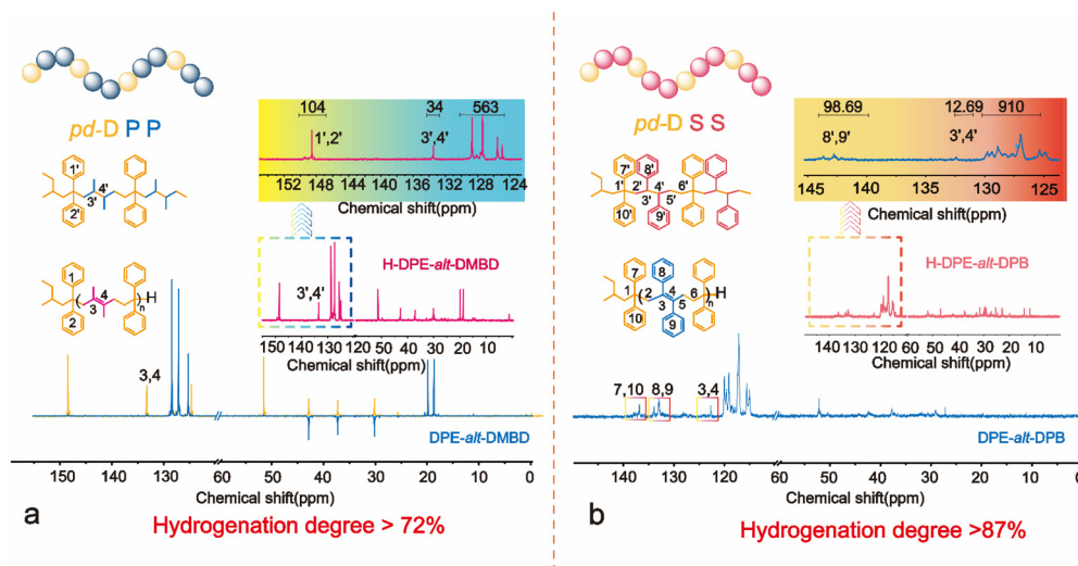
Fig. 3 IG- ^{13}\text{C} NMR spectra of alternating polymers and periodic polymers: (a) for the copolymer of DPE with DMDB and (b) for the copolymer of DPE with DPB.
