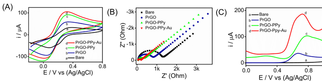
Fig. 4 (A) CV responses of different modified electrodes: (a) bare, (b) PrGO, (c) PrGO-PPy, and (d) PrGO-PPy-Au obtained in a solution containing 2 \text{ mM } K_3[Fe(CN)_6] and 0.1 \text{ M KCl} . The potential was applied between -0.1 \text{ V} and 0.8 \text{ V} at a scan rate of 100 \text{ mV s}^{-1} . (B) Nyquist plots obtained for the SPCE and various modified electrodes in an aqueous solution of 2 \text{ mM } K_3[Fe(CN)_6] and 0.1 \text{ M KCl} . (C) SWV responses of various electrodes: (a) bare, (b) PrGO, (c) PrGO-PPy, and (d) PrGO-PPy-Au recorded at a methotrexate (MTX) concentration of 25 \text{ } \mu\text{M} .
