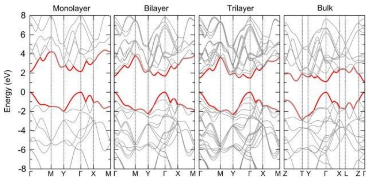
Figure 9: The calculated electronic band structures for monolayer, bilayer, trilayer, and bulk black phosphorus (BP) reveal how the electronic properties evolve as the thickness increases, from a single layer to the bulk material, reproduced from ref [77] with permission from IOP Publishing, copyright 2014.
