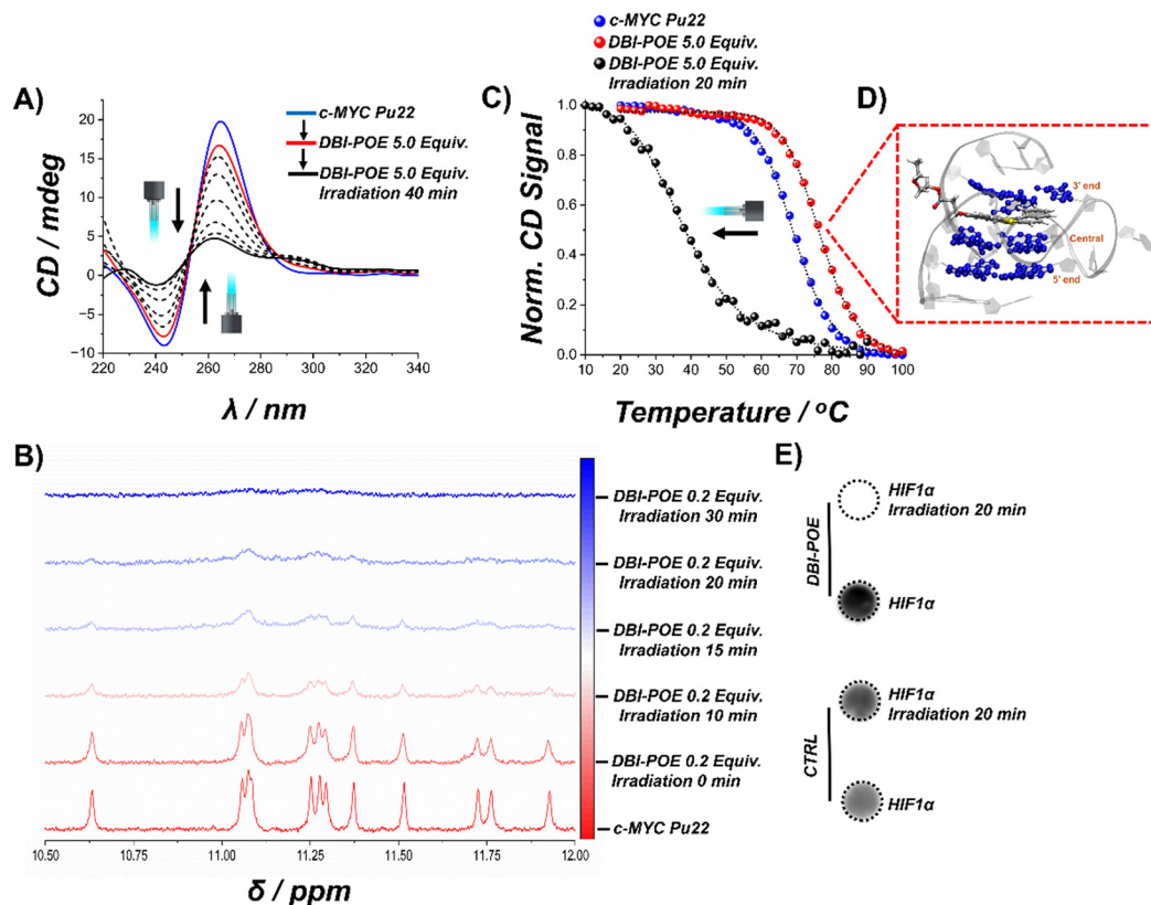
Fig. 4 (A) CD spectra of c -MYC Pu22 recorded in the absence and presence of DBI-POE. Measurements were performed using c -MYC Pu22 = 2 \mu\text{M} and DBI-POE = either 0 or 10 \mu\text{M} in 50 mM Tris buffer (pH 6.8) containing 100 mM KCl. (B) ^1\text{H} NMR spectra of c -MYC Pu22 recorded in the absence and presence of DBI-POE. Measurements were performed using c -MYC Pu22 = 200 \mu\text{M} and DBI-POE = either 0 or 40 \mu\text{M} in 50 mM Tris buffer (pH 6.8) containing 100 mM KCl. (C) CD-based melting profiles of c -MYC Pu22 recorded in the absence and presence of DBI-POE, plotted at the CD maximum at 264 nm. Measurements were performed using c -MYC Pu22 = 2 \mu\text{M} and DBI-POE = either 0 or 10 \mu\text{M} in 50 mM Tris buffer (pH 6.8) containing 5 mM KCl. (D) Representative MD structure of DBI-POE stable poses from the dbSCAN clustering of the last 1 \mu\text{s} of the MD production. (E) Dot blot assay was performed using HIF-1 \alpha = 8 \mu\text{M} and DBI-POE = either 0 or 8 \mu\text{M} in 10 mM Tris buffer (pH 7.4) containing 100 mM KCl. (A–C) Irradiation was carried out at 485 \pm 20 nm at an irradiance of 10 \text{ mW cm}^{-2} over various time intervals. (E) Irradiation was carried out at 460–495 nm for 20 min. DMSO was used as a control in all experiments.
