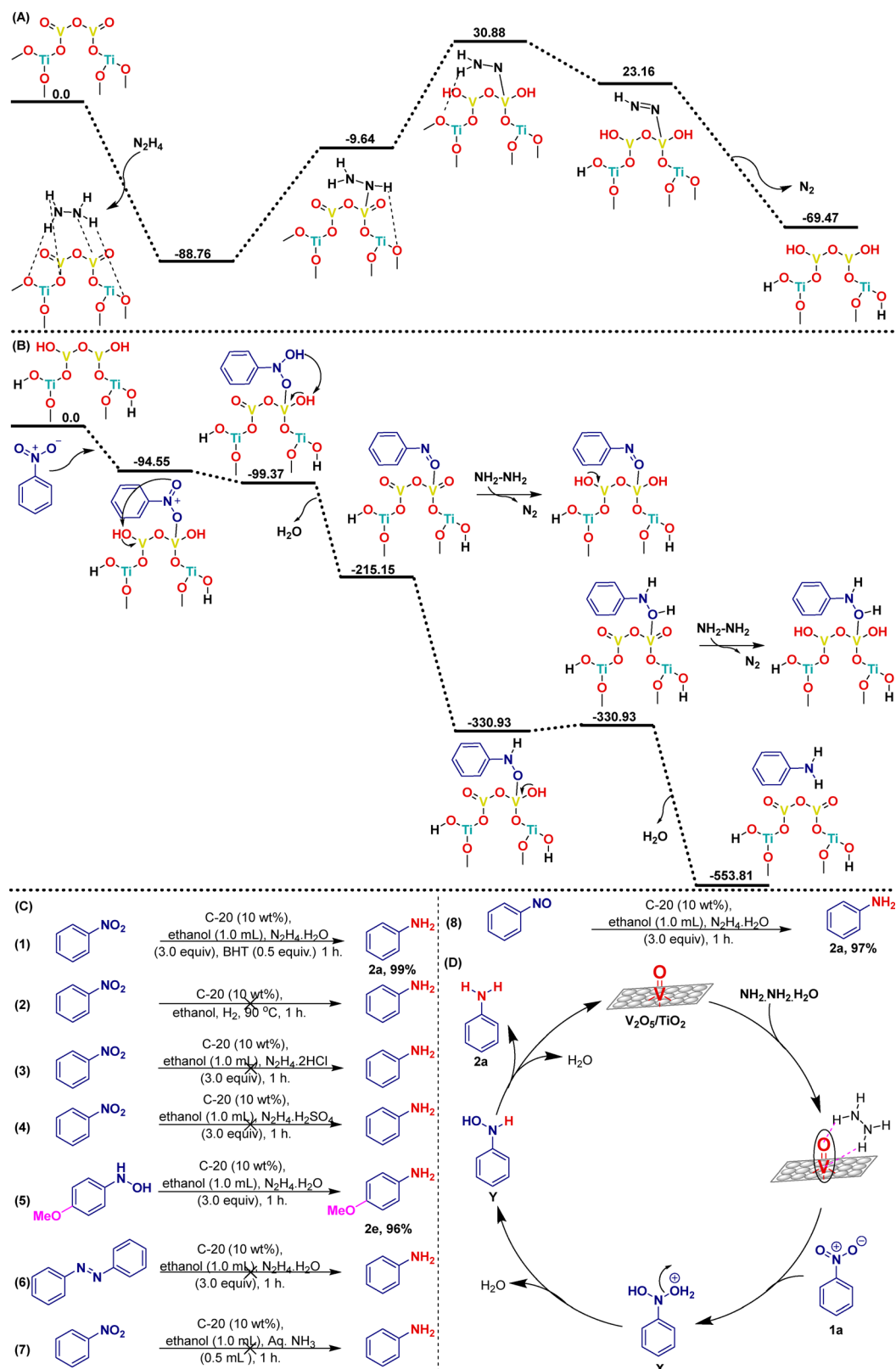
Fig. 7 (A) Reaction energy profile of dehydrogenation of \text{N}_2\text{H}_4 over the \text{V}_2\text{O}_5/\text{TiO}_2 (001) surface (reaction energies are labelled in kJ mol -1 ), (B) reaction energy profile of nitrobenzene reduction to aniline over hydrogenated \text{V}_2\text{O}_5/\text{TiO}_2 (001) (reaction energies are labelled in kJ mol -1 ), (C) control experiments and (D) plausible mechanism.
