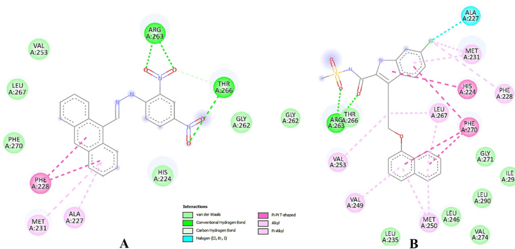
Fig. 17 2D interaction diagrams of (A) the selected molecule P1 and (B) experimentally co-crystallised inhibitor 5WL docked within the binding domain of the Mcl-1 protein.
