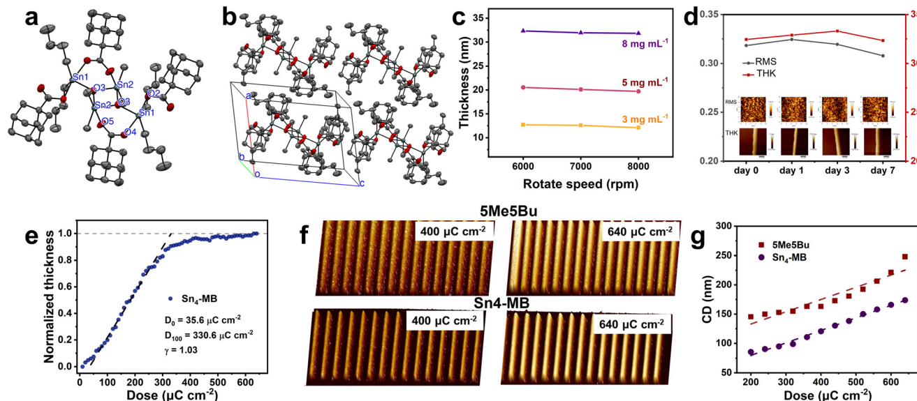
Fig. 1 (a) and (b) Single crystal structures of Sn 4 -MB. The hydrogen atoms were omitted for clarity; (c) thickness of films obtained from different concentrations of Sn 4 -MB precursor solutions at different rotational speeds; (d) time-dependent variation in surface roughness (RMS) and film thickness (THK) of Sn 4 -MB films at days 0, 1, 3, and 7 after spin-coating. Insets show AFM surface topography (top row) and cross-sectional profiles (bottom row), corresponding to the same time points from left to right; (e) contrast curves of Sn 4 -MB; (f) AFM images of L/3S dense line patterns (100 nm pitch) generated from Sn 4 -MB and 5Me5Bu resists under area-exposure at electron-beam doses of 400 and 640 μC cm -2 ; (g) periodic line CD of Sn 4 -MB and 5Me5Bu films under area-exposure as a function of exposure dose.
