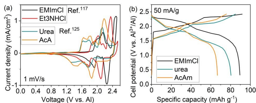
Figure 13. a) CV curves of \text{Al}/\text{expanded graphite} cells with \text{AlCl}_3/[\text{EMIm}]\text{Cl} and \text{AlCl}_3/\text{Et}_3\text{NHCl} electrolytes 117 and \text{Al}/\text{natural graphite} cells employing \text{AlCl}_3/\text{urea} and \text{AlCl}_3/\text{AcA} electrolytes 125 (molar ratio 1.5:1) at a scan rate of 1\text{ mV/s} . b) Charge/discharge profiles of \text{Al}/\text{natural graphite} cells with \text{AlCl}_3/[\text{EMIm}]\text{Cl} , \text{AlCl}_3/\text{urea} and \text{AlCl}_3/\text{AcA} electrolytes (molar ratio 1.5:1) at a current density of 50\text{ mA g}^{-1} . 125 Adapted with permission from Elsevier 117 . Copyright 2019. Adapted with permission from Wiley 125 . Copyright 2021.
