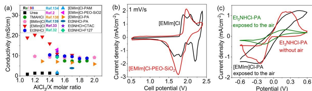
Figure 15. a) Ionic conductivity of various \text{AlCl}_3/\text{X} electrolytes. X = [EMIm]Cl (10–20 mS cm -1 ), TMAHCl (average ~7.5 mS cm -1 ), \text{Et}_3\text{NHCl} (~9.6 mS cm -1 ), [BMIm]Cl (~9.4 mS cm -1 ), and urea (~1.3 mS cm -1 ) were measured at 25 °C. 98 [EMIm]Cl-PAM (1.66×10 -3 S cm -1 , measured at 20 °C) is gel polymer electrolyte made from \text{AlCl}_3 complexed acrylamide and \text{AlCl}_3/[\text{EMIm}]\text{Cl} (1.5:1). 134 [EMIm]Cl-PEO-SiO 2 (13 mS cm -1 ) is gel polymer electrolyte made from PEO, \text{AlCl}_3/[\text{EMIm}]\text{Cl} (1.5:1) and an additive-fumed SiO 2 . 2 [EMIm]Cl-PA (5.89 to 7.24 mS cm -1 , measured at room temperature) and \text{Et}_3\text{NHCl} -PA (3.86 mS cm -1 , measured at 25 °C) is PA-based gel polymer electrolyte made with \text{AlCl}_3/[\text{EMIm}]\text{Cl} (2:1 to 1.3:1) 138 and \text{AlCl}_3/\text{Et}_3\text{NHCl} (1.7:1) 139 , respectively. \text{AlCl}_3/\text{Et}_3\text{NHCl} (1.5:1) add CTAC (12.06 mS cm -1 ) 33 and F127 (9.31 mS cm -1 ) 32 are named \text{Et}_3\text{NHCl} +CTAC and \text{Et}_3\text{NHCl} +F127, respectively. b) CV curves of Al//natural graphite cells with \text{AlCl}_3/[\text{EMIm}]\text{Cl} and \text{AlCl}_3/[\text{EMIm}]\text{Cl} -PEO-SiO 2 electrolytes showing anions intercalation at a scan rate of 1 mV s -1 . Adapted from Leung, O. M. et al, Adv. Energy Mater. 2 . Licensed under CC BY 3.0. ©2024 John Wiley and Sons. c) CV curves of Al//natural graphite cells with \text{AlCl}_3/[\text{EMIm}]\text{Cl} -PA 138 (not mentioning the scan rate) and \text{AlCl}_3/\text{Et}_3\text{NHCl} -PA 139 (without air not mentioning the scan rate, and after being exposed to the air for 10 min at a scan rate of 1 mV s -1 ) presenting Al plating/stripping. Adapted with permission from Elsevier 138 . Copyright 2021. Adapted with permission from American Chemical Society 139 . Copyright 2021.
