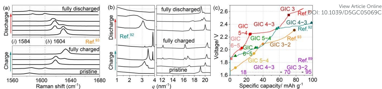
Figure 11. a) Selected in-situ Raman spectra of the graphite electrode recorded during charge/discharge at 50 mA g -1 . 93 b) Selected SAXS (left) and WAXS (right) profiles of the first cycle along with charge/discharge at 50 mA g -1 . 92 c) The relative specific capacity across intercalation stages during the first cycle based on publication: galvanostatic charging curve (25 mA g -1 ) of Swagelok type cell 89 and PEEK self-made cell 92 with AlCl 3 /[EMIM]Cl (1.5:1) electrolyte, galvanostatic charging curve (50 mA g -1 ) of pouch cell with AlCl 3 /[EMIM]Cl (1.7:1) at -10 °C 91 , and galvanostatic charging curve (50 mA g -1 ) of pouch cell with AlCl 3 /urea (1.3:1) electrolyte 93 . Adapted from Elia, G. A. et al., Adv. Funct. Mater. 89 Licensed under CC BY. ©2020 Wiley. Adapted with permission from author. Copyright 2018 91 . Adapted from Greco, G. et al., Small Methods 92 . Licensed under CC BY 3.0. ©2021 Wiley. Adapted with permission from author 93 . Copyright 2017.
