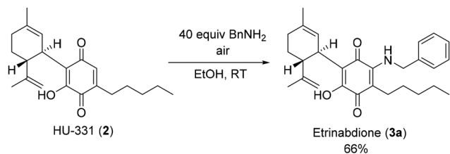
Scheme 2 Synthesis of Etrinabdone ( 3 ) via treatment of 2 with a large excess of benzylamine and subsequent aerobic oxidation with air.
