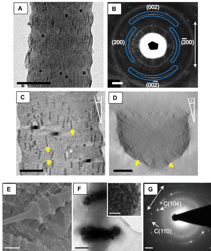
Fig. 23 Xu et al. 114 studied the effect of confinement on crystal growth in collagen by using XRD to determine the voids in collagen are cylindrical pores with diameters of around 2 nm. (A) and (B) In addition to HAp (not shown here), they also demonstrated the concept of confinement with lepidocrocite, \gamma -FeOOH, which also has an anisotropic lattice structure (orthorhombic). (C) and (D) Tomographic reconstruction with an averaging of ten y - and z -slices. The orientations of some \gamma -FeOOH platelets are highlighted by yellow arrows in (C). (E)–(G) They found that \text{CaCO}_3 produced a mix of calcite and vaterite (not shown here), and with a sustained granular texture, they showed no preferential orientation. Interestingly, their intrafibrillar calcite produced orthogonal bulges similar to what we had observed in our first \text{CaCO}_3 collagen study. It would be interesting if someone could produce intrafibrillar aragonite, because it normally grows as anisotropic needles. Reproduced from ref. 114, Copyright © 2020, The Authors.
