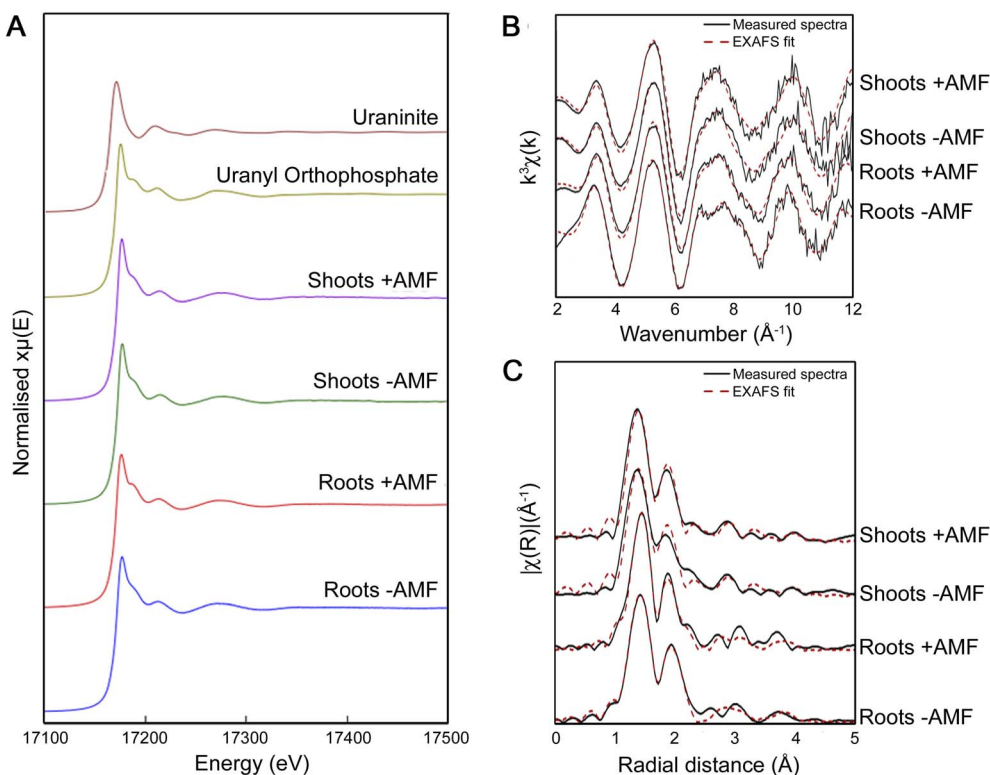
Fig. 7 (A) Bulk U L_{3\alpha} edge XANES shoot and root spectra for U-dosed non-mycorrhizal (–AMF) and mycorrhizal (+AMF) specimens, and for uranyl orthophosphate ( \text{U(VI)} ) and uranyl orthophosphate ( \text{U(VI)} ) standards. The \text{U(VI)} edge position from uranyl orthophosphate occurs at 17171 eV. (B and C) U EXAFS k -space spectra (B) and Fourier Transform spectra (C) acquired from L_{3\alpha} -edge analysis of shoot and root spectra for U-dosed non-mycorrhizal (–AMF) and mycorrhizal (+AMF) specimens. Black solid lines represent collected spectra while the red dashed line indicates the modelled best-fit spectra. This figure suggests that the dominant U oxidation state in all of the shoot and root section treatments is \text{U(VI)} , akin to uranyl orthophosphate, irrespective of AMF colonisation status.
