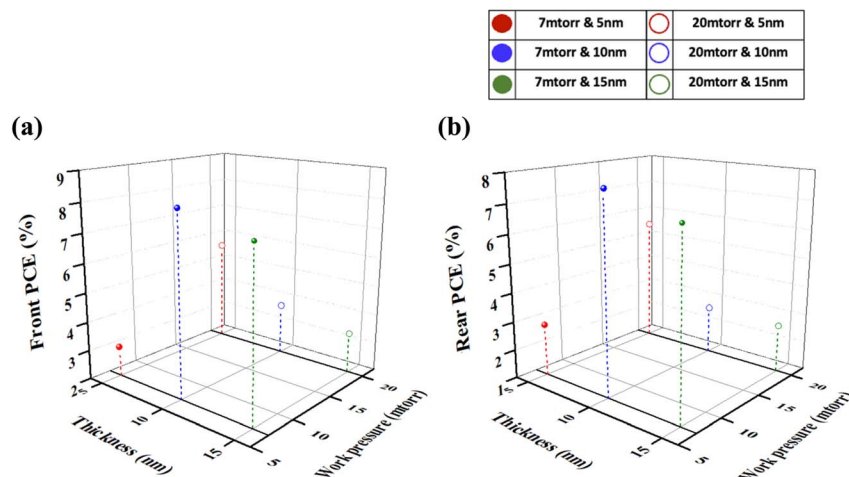
Fig. 5 For bifacial devices with sputtered buffer layers, measured under AM 1.5 G 1 sun illumination, the performance with different SnO 2 thicknesses and working pressures: (a) front-side efficiency and (b) rear-side efficiency.
