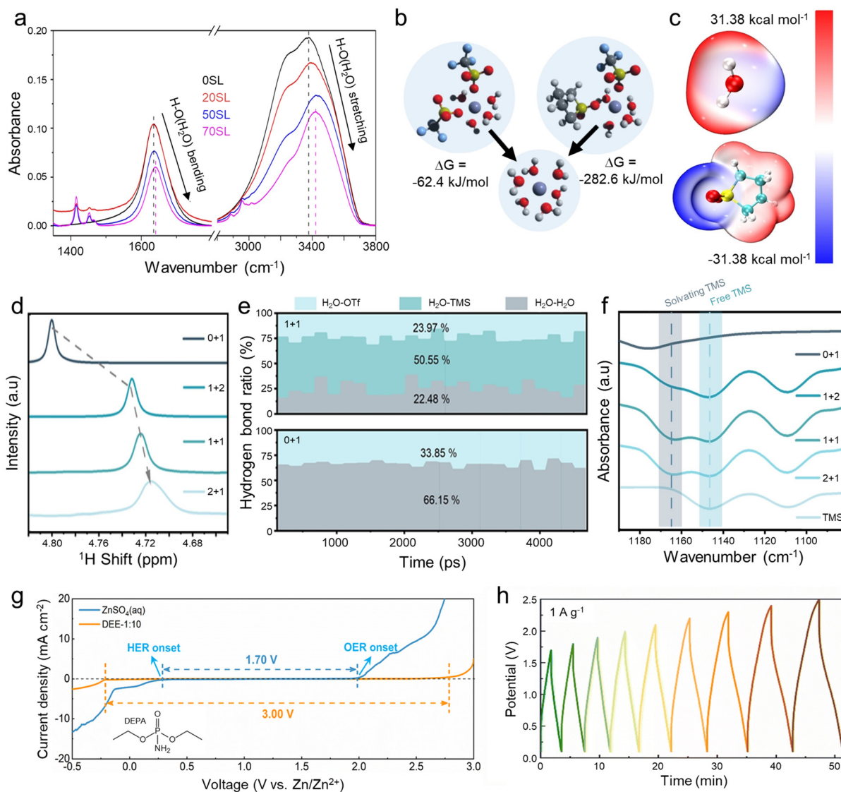
Fig. 3 Design principles of electrolytes with widened ESW guided by DES chemistry. (a) FTIR spectral evolution of electrolytes with SL. (b) DFT-computed reaction energies to form fully hydrated \text{Zn}^{2+} from other cluster types (left: \text{Zn}^{2+} \cdot 4\text{H}_2\text{O} \cdot 2\text{OTf}^- , right: \text{Zn}^{2+} \cdot 4\text{H}_2\text{O} \cdot 1\text{OTf}^- \cdot 1\text{SL} ). Reproduced with permission from ref. 89. Copyright 2023, Springer Nature. (c) Electrostatic potential maps of TMS and \text{H}_2\text{O} molecule. (d) NMR spectra with varying TMS content. (2 M \text{Zn}(\text{OTf})_2 concentration is maintained, ratio of TMS to \text{H}_2\text{O} is 0 : 1, 1 : 2, 1 : 1 and 1 : 2) (e) Different types of hydrogen bonds ratio in MD simulation of 1 + 1 and 0 + 1, (f) FTIR spectra of pure TMS, 0 + 1, 1 + 2, 1 + 1 and 2 + 1. Reproduced with permission from ref. 90. Copyright 2023, Wiley-VCH. (g) LSV curves of Zn-SS cells using a DES electrolyte containing DEPA and a \text{ZnSO}_4 -based aqueous electrolyte at 1 \text{ mV s}^{-1} . The inset presents the chemical structure of DEPA. (h) GCD curves of Zn-ion hybrid capacitor from 0.1 V to 2.5 V. Reproduced with permission from ref. 92. Copyright 2024, The Royal Society of Chemistry.
