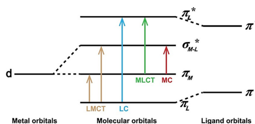
Fig. 1 Simplified diagram illustrates different types of electronic transitions in photoluminescent MOF. (Reproduced from ref. 34 Copyright 2025 with permission from Elsevier).
