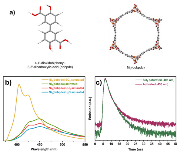
Fig. 10 (a) Structure of linker and \text{Ni}_2(\text{dobpdc}) , (b) selective response of \text{Ni}_2(\text{dobpdc}) towards \text{SO}_2 , and (c) decay-time of activated and \text{SO}_2 saturated samples (reproduced from ref. 67).
