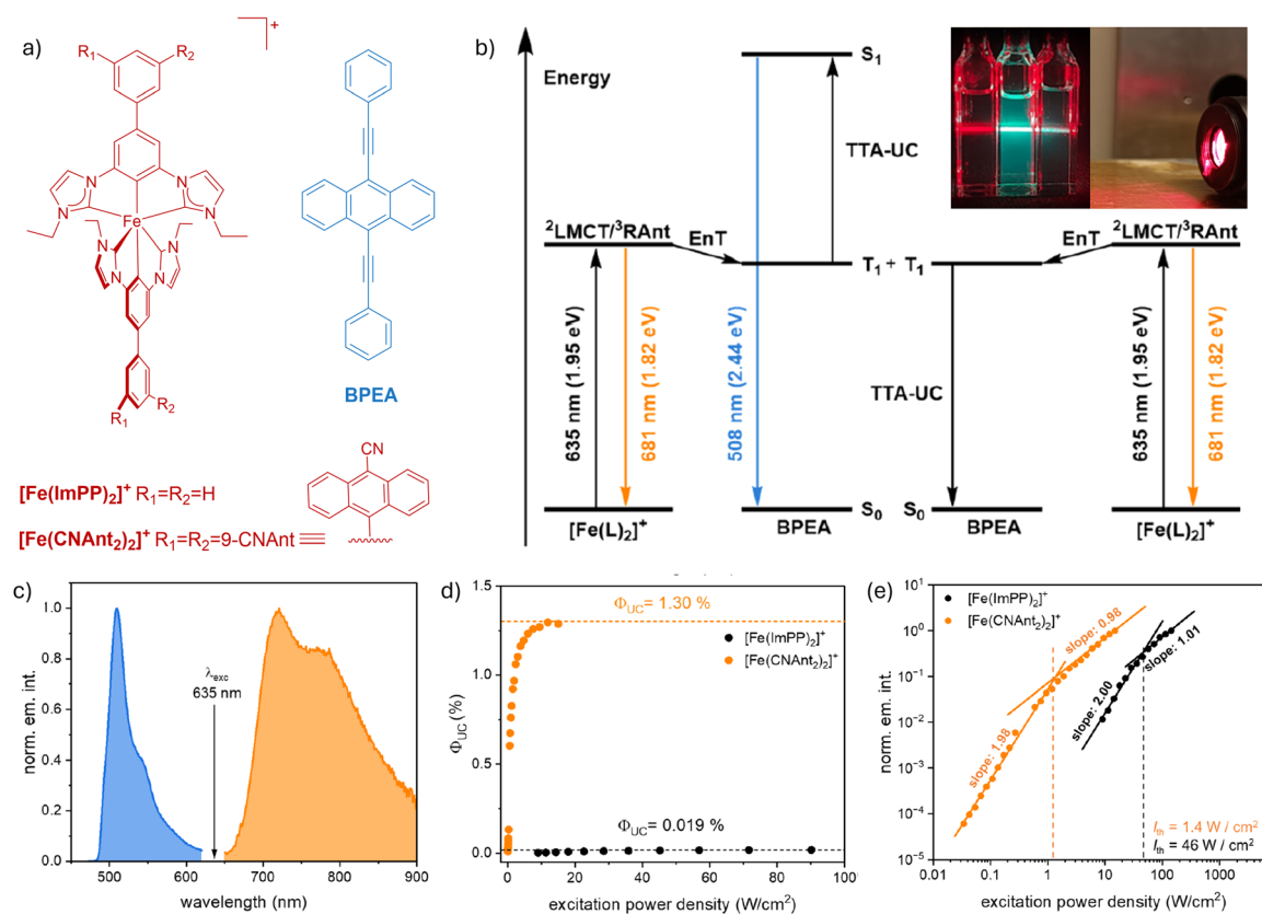
Fig. 4 Red-to-green upconversion sensitized by [\text{Fe}(\text{ImPP})_2]^+ and [\text{Fe}(\text{CNAnt})_2]^+ with 9,10-bis(phenylethynyl)anthracene (BPEA) as the annihilator. (a) Molecular structures of [\text{Fe}(\text{ImPP})_2]^+ , [\text{Fe}(\text{CNAnt})_2]^+ and BPEA. (b) Energy-level diagram of sTTA-UC with [\text{Fe}(\text{ImPP})_2]^+ and [\text{Fe}(\text{CNAnt})_2]^+ as the photosensitizers and BPEA as the annihilator. Inset: Photographs of the samples containing only [\text{Fe}(\text{CNAnt})_2]^+ without BPEA (left) and the upconverting pairs [\text{Fe}(\text{CNAnt})_2]^+ /BPEA (middle) as well as [\text{Fe}(\text{ImPP})_2]^+ /BPEA (right) under 635 nm CW-laser excitation (laser power = 1.0 W). (c) Normalized luminescence spectra recorded from a [\text{Fe}(\text{CNAnt})_2]^+ solution (orange) and a solution containing the [\text{Fe}(\text{CNAnt})_2]^+ /BPEA pair (blue) in deaerated 1,2-dichloroethane at 20 °C following CW-laser excitation at 635 nm. (d) Upconversion luminescence quantum yield \Phi_{\text{UC}} obtained from the upconversion pairs [\text{Fe}(\text{CNAnt})_2]^+ /BPEA (orange) and [\text{Fe}(\text{ImPP})_2]^+ /BPEA (black) as a function of the excitation power density at 635 nm. (e) Log-log plots of the upconversion luminescence intensity as a function of the excitation power density, giving a threshold I_{\text{th}} value of \sim 1.4 \text{ W cm}^{-2} for the [\text{Fe}(\text{CNAnt})_2]^+ /BPEA pair (orange) and \sim 46 \text{ W cm}^{-2} for the [\text{Fe}(\text{ImPP})_2]^+ /BPEA pair (black). 31,130 (b)–(e) Reproduced under terms of the CC-BY-NC-ND license from ref. 166. Copyright 2025, American Chemical Society.
