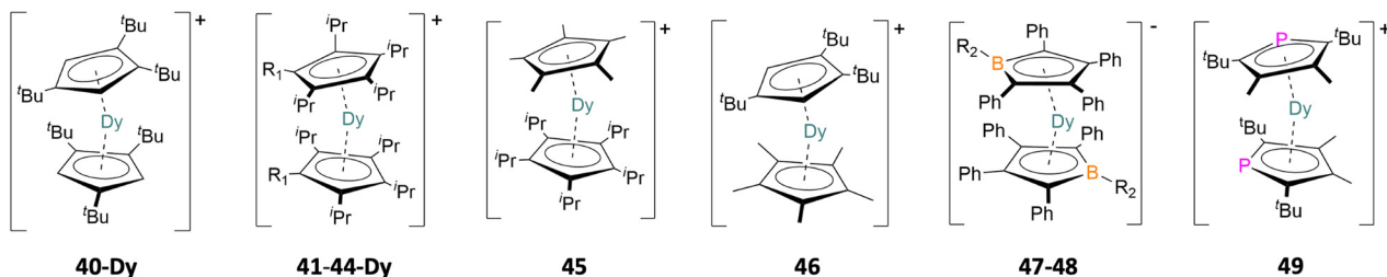
Fig. 6 Examples of the pseudo-linear dysprosocenium ions from [Dy(Cp ttt ) 2 ][B(C 6 F 5 ) 4 ] ( 40-Dy ), [Dy(Cp Pr ) 2 ][B(C 6 F 5 ) 4 ] ( 41 , R 1 = H), [Dy(Cp Pr ,Me c ) 2 ][B(C 6 F 5 ) 4 ] ( 42 , R 1 = Me), [Dy(Cp Pr ,Et c ) 2 ][B(C 6 F 5 ) 4 ] ( 43 , R 1 = Et), [Dy(Cp Pr ) 2 ][B(C 6 F 5 ) 4 ] ( 44-Dy , R 1 = i Pr), [Dy(Cp Pr )(Cp*)][B(C 6 F 5 ) 4 ] ( 45 ), [Dy(Cp ttt )(Cp*)][Al(OC(CF 3 ) 3 ) 4 ] ( 46 ), [K(18-crown-6)(THF) 2 ][Dy(BC 4 Ph 5 ) 2 ] ( 47 , R 2 = Ph), [K(2.2.2)][Dy(BC 4 Ph 4 Pip) 2 ] ( 48 , R 2 = NC 5 H 10 ) and [Dy(PC 4 tBu,Me 2 ) 2 ][Al(OC(CF 3 ) 3 ) 4 ] ( 49 ). 59–62,67–69
