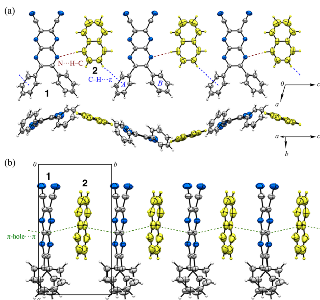
Fig. 3 a) Top (viewed along the b -axis) and side (rotated 90^\circ ) views of the packing structure with a layered arrangement, and b) columnar arrangement along the b -axis (viewed along the c -axis) of Y.
