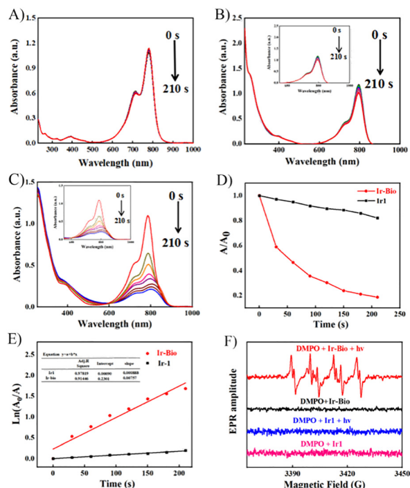
Fig. 2 (A) UV absorption spectra of ICG at different illumination times (405 nm, 20 mW cm -2 ); (B) ICG + Ir1 + light; (C) ICG + Ir-Bio + light; (D) the attenuation curve of ICG at 790 nm when Ir1 or Ir-Bio (18 μM) is present under different illumination times, data in DMSO : H 2 O (v : v = 1 : 99); (E) 1 O 2 kinetic generation curve of Ir1 / Ir-Bio ; (F) EPR signals of Ir1 and Ir-Bio (0.1 mM) and DMPO (100 mM) under light and dark conditions in DMSO.
