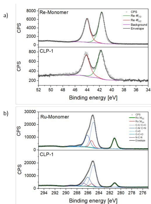
Figure 3: Detailed XPS scans of CLP-1 and Monomers. Re 4f (top) and C1s together with Ru 3d 5/2 (bottom).
