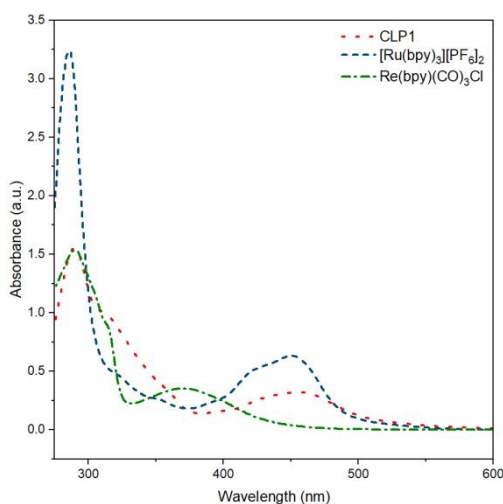
Figure 2: UV-Vis spectra of polymer CLP-1 (red, dot), and complexes [\text{Ru}(\text{bpy})_3][\text{PF}_6]_2 (blue, dash) and \text{Re}(\text{bpy})(\text{CO})_3\text{Cl} in MeCN (green, dash-dot).
