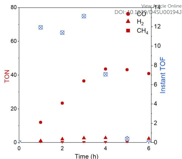
Figure 5: Turnover number (TON) and instant turnover frequency (Instant TOF) of CO 2 reduction reaction over the time course of 6 h with CLP-1.
