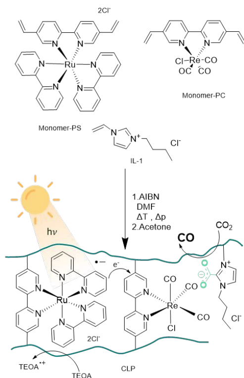
Figure 1: Schematic representation of monomers used for the radical polymerisation of crosslinked polymers (CLP) with AIBN (azobisisobutyronitrile) towards a polymer framework for photocatalytic CO 2 reduction.
