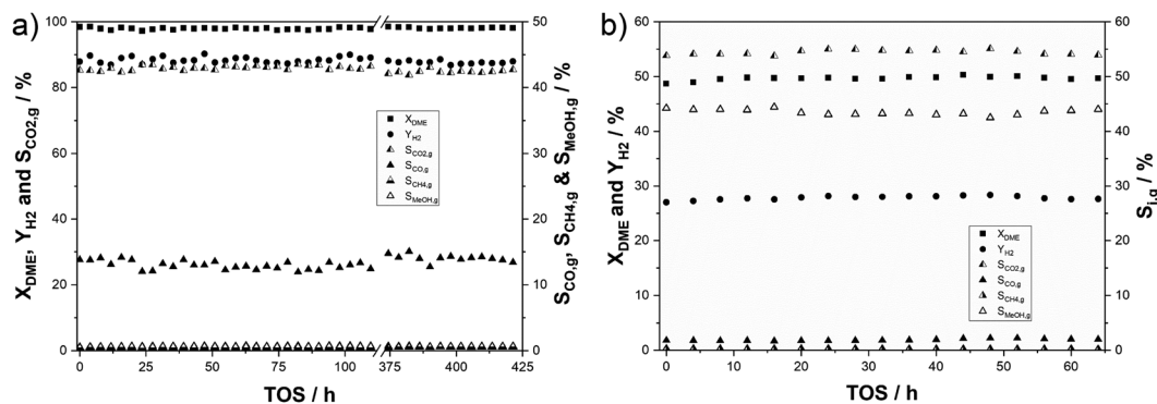
Fig. 5 DME conversion, hydrogen yields and C 1 selectivities of (a) the physical mixture of 36 g In 2 O 3 /ZrO 2 (3 wt% indium content) and 9 g \gamma -Al 2 O 3 ( t_{\text{reaction}} = 425 h; GHSV = 550 h -1 ; p = 2 bar) and (b) the physical mixture of 3 g In 2 O 3 /ZrO 2 (3 wt% indium content) and 3 g \gamma -Al 2 O 3 ( t_{\text{reaction}} = 64 h; GHSV = 2500 h -1 ; p = 2 bar); molar ratio of n_{\text{H}_2\text{O}} : n_{\text{DME}} : n_{\text{N}_2} = 5 : 1 : 1.5 ; T_{\text{SRD}} = 350 °C) and (b) the physical mixture of 3 g In 2 O 3 /ZrO 2 (3 wt% indium content) and 3 g \gamma -Al 2 O 3 ( t_{\text{reaction}} = 64 h; GHSV = 2500 h -1 ; p = 2 bar); molar ratio of n_{\text{H}_2\text{O}} : n_{\text{DME}} : n_{\text{N}_2} = 5 : 1 : 1.5 ; T_{\text{SRD}} = 350 °C).
