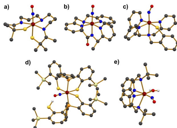
Fig. 2 Crystal structures of Fe–NO complexes, (a) [FeS 2 Me 2 N 3 (Pr,Pr)(NO)] + (7), (b) [Fe(MePcPy 3 )(NO)] 2+ (10), (c) [Fe(N3PyS)(NO)] + (13), (d) [Fe(T Me PS 2 )(T Me PS 2 H)(NO)] (16), and (e) [Fe(TBDAP)(NO)(H 2 O)] 2+ (20) (dark grey, C; blue, N; red, O; yellow, S; scarlet, Fe).
