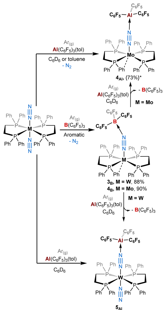
Scheme 2 Reactivity of \text{ML}_2(\text{N}_2)_2 ( \text{M} = \text{W}, \text{Mo} ; \text{L} = \text{dppe} ) complexes with \text{B}(\text{C}_6\text{F}_5)_3 and \text{Al}(\text{C}_6\text{F}_5)_3(\text{tol}) under an argon atmosphere. {The yield in brackets followed by a star*} represents the NMR yield. The other complexes ( \text{L} = \text{depe} or \text{dmpe} ) reacted similarly as under a dinitrogen atmosphere (see Scheme 1).
