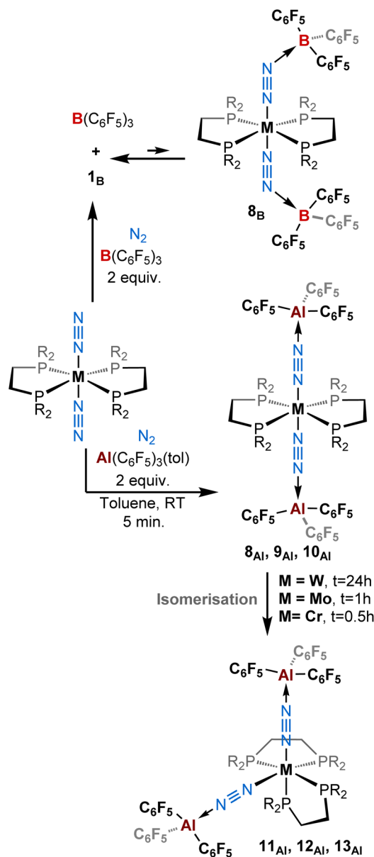
Scheme 3 Reactivity of [\text{ML}_2(\text{N}_2)_2] ( \text{M} = \text{W}, \text{Mo}, \text{Cr} ; \text{L} = \text{depe}, \text{dppe}, \text{dmppe} ) complexes with (top) two equivalents of \text{B}(\text{C}_6\text{F}_5)_3 and (bottom) two equivalents of \text{Al}(\text{C}_6\text{F}_5)_3(\text{tol}) under a dinitrogen atmosphere.
