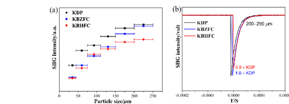
Fig. 3 (a) Powder SHG measurements of KDP, KBZFC, and KBHFC at 1064 nm. (b) SHG signals from KBZFC and KBHFC compared with benchmark KDP at 200–250 \mu\text{m} .
