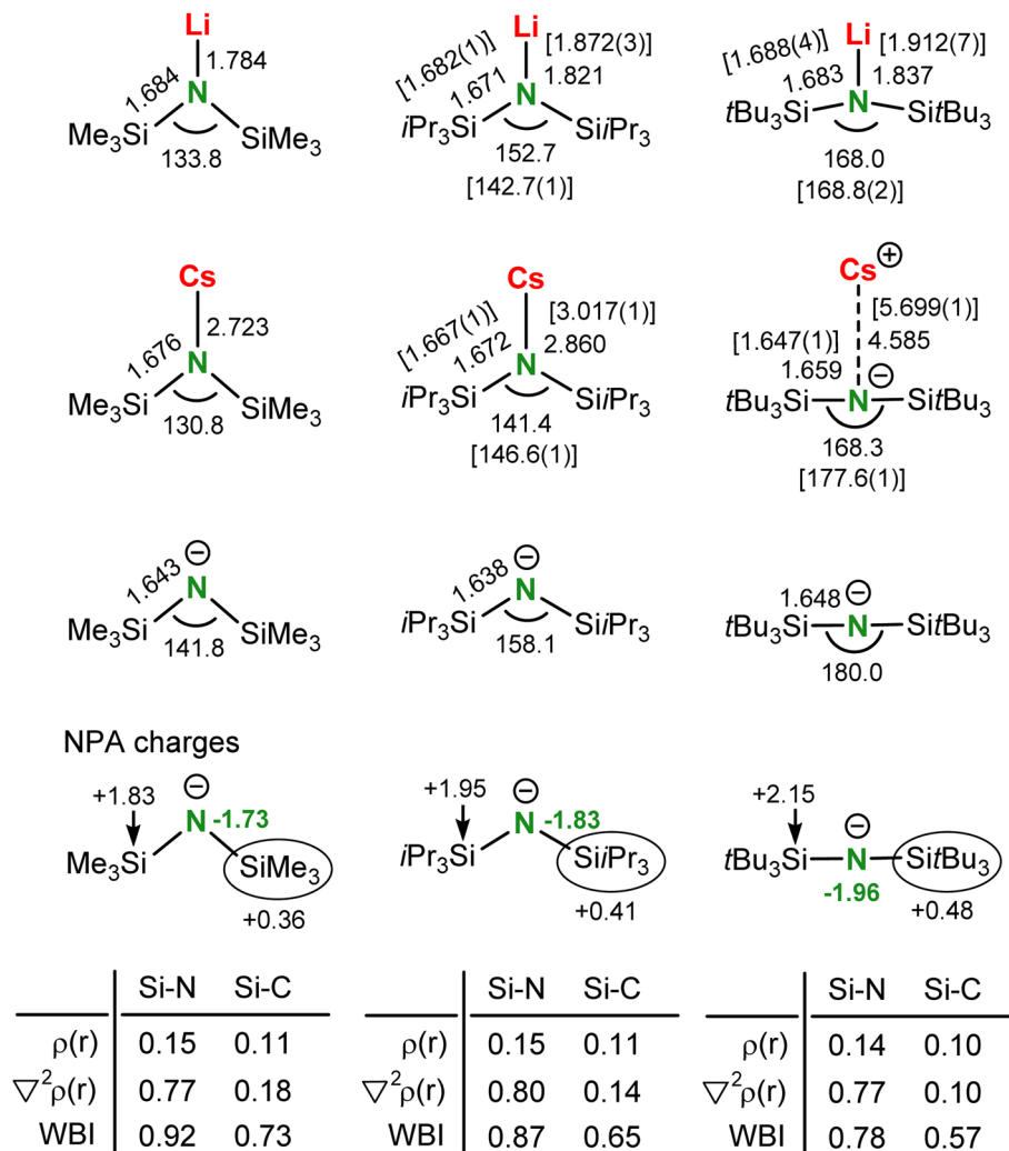
Scheme 5 Comparison of DFT-optimized Li and Cs amide complexes and the free anions Me N - , iPr N - and tBu N - (B3PW91/def2tzvp including GD3BJ dispersion corrections) showing distances (Å), angles (°), Wiberg bond indices (WBIs) and values for \rho(r) and the Laplacian \nabla^2\rho(r) in the bond-critical point (a.u.). Values for crystal structures are given between square brackets.
